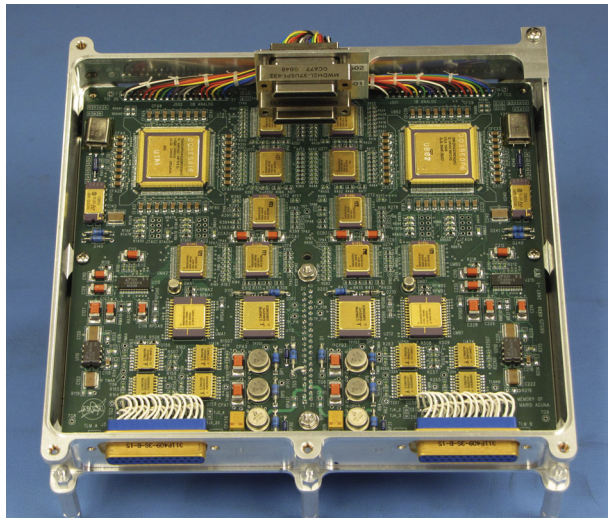
Fig. 22 Fluxgate magnetometer digital card in its frame prior to assembly. The digital system is dual hardware redundant (note symmetry) and only one side is powered at a time; the other is cold spared
