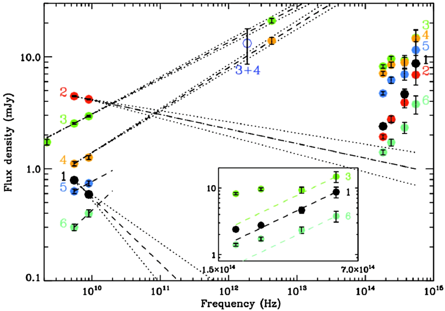
Fig. 14 Evolution of the radio to OIR SED during the soft to hard state transition as the jets reform, and become optically thick. The numbers (and associated colors) refer to sequential epochs, and the dashed lines correspond to the extrapolation of the radio spectra. Inset : zoom of the OIR spectra # 1, 3 and 6. From Corbel et al. (2013)
