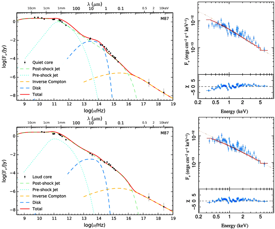
Fig. 16 An outflow-dominated model fit to the SED of M87, where all data are from within a 0.4 arcsec aperture radius (32 pc). The top panel shows the result for the quiescent state, the bottom panel for the active one. The X-ray spectrum used in the model for both states is the 2002 Chandra spectrum, the fit for which is shown as a separate plot. The data are fit using the model in Markoff et al. (2005) that is also applied to XRBs, and a location of the break implies an acceleration region of 10s of r_g , similar to XRBs as well. From Prieto et al. (2016)
