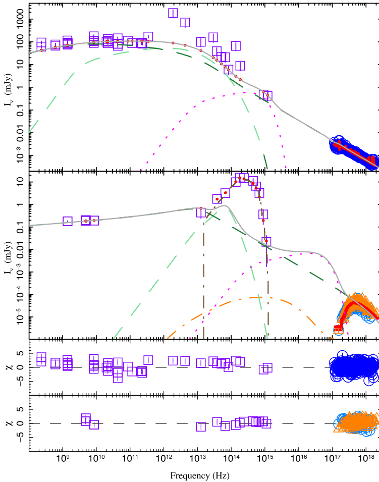
Fig. 17 Best joint-fit model with all physical free parameters tied to SEDs of similar accretion power (based on L_X/L_{\text{Edd}} from the LLAGN M81) (top) and hard state XRB V404 Cyg (bottom). Lines show the individual model components (light green/dashed: thermal synchrotron, dark green/dashed: non-thermal synchrotron, orange/dashed-dotted: synchrotron self-Compton, magenta/dotted: multicolor blackbody disk, and gray/dashed-dotted: stellar component in the case of V404), all absent absorption. The gray/solid line shows the total model, while the red/solid line and dots show the model after forward folding through detector space, including absorption. The IR/optical part of the M81 SED also includes a galactic stellar and dust contribution (not fitted). The spectral break in both sources implies a particle acceleration region in the jets starting at 300r_g . From Markoff et al. (2015)
