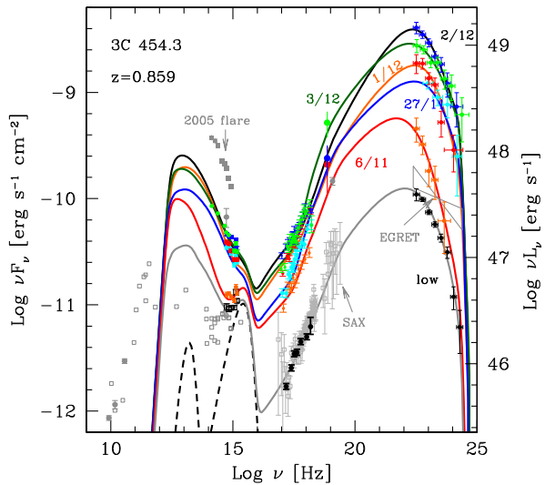
Fig. 2 Spectral energy distributions of the FSRQ 3C454.3 during different activity states in 2012 (colored) and a quiescent phase (gray). The data clearly show the typical “double humped” shape of the SED. Curves show the result of a one-zone leptonic emission model. The reader can appreciate the extreme variability, especially in the \gamma -ray band. From Bonnoli et al. (2011)
