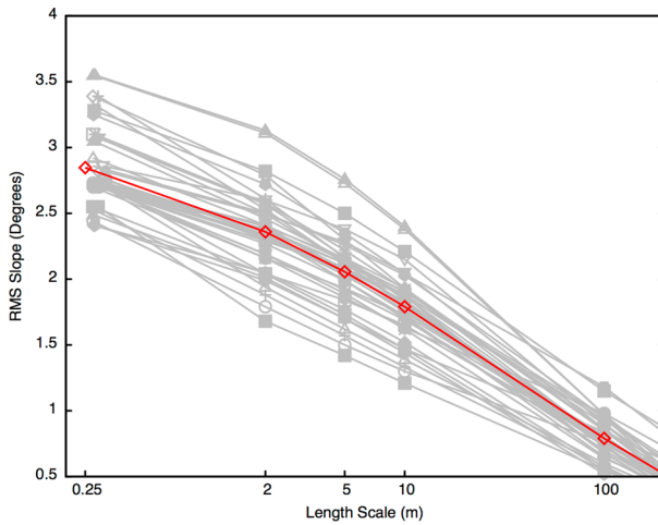
Fig. 23 Bidirectional RMS slope versus baseline length of HiRISE images in ellipse E9 from photogrammetry ( red is the average). RMS slope varies with baseline length from <1^\circ at 100 m to 2.5\text{--}3.5^\circ at 25 cm. The photogrammetry derived RMS slope at 100 m length scale compares favorably with MOLA extrapolated RMS slopes at the same scale (see Sect. 7.6.1). In addition, RMS slopes at 25 cm are only 20–25 % greater than that at 2 m, suggesting that only a fraction of 1 % of the surface exceeds the 15^\circ limit to successfully deploy the instruments. Bidirectional slopes are produced by averaging the brightness values over each length scale and then running the photogrammetry algorithm on the downsampled image (Beyer et al. 2016). Bidirectional slopes are \sqrt{2} lower than adirectional slopes
