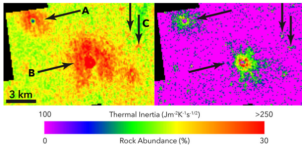
Fig. 15 Comparison of THEMIS thermal inertia map ( left ) and HiRISE derived rock abundance derived in Sect. 7.5 ( right ) illustrating the excellent correlation between both mapping products. A : example of a rocky ejecta blanket showing similar extent in the visible and infrared data; B : example of a rocky ejecta blanket that is smaller in images than in the infrared (see text for discussion); C : example of smaller and more degraded rocky ejecta blankets with faint but noticeable signatures in the thermal inertia and rock abundance maps
