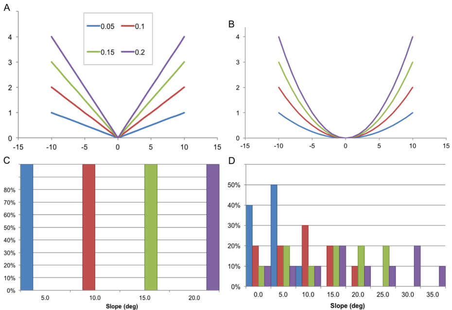
Fig. 29 Theoretical shape models and the resulting slopes for conical and parabolic shaped craters as observed in DEMs. Cross-sections of conical- (A) and parabolic-shaped (B) craters with d/D = 0.05, 0.10, 0.15, and 0.20 with dimensionless axes of height and length. Histograms of the slopes in the theoretical cross-sections, conical (C) and parabolic (D). Note that slopes for conical and parabolic shape craters with d/D of 0.05 are <6^\circ and <11^\circ , respectively, and thus less than the 15^\circ engineering constraint
