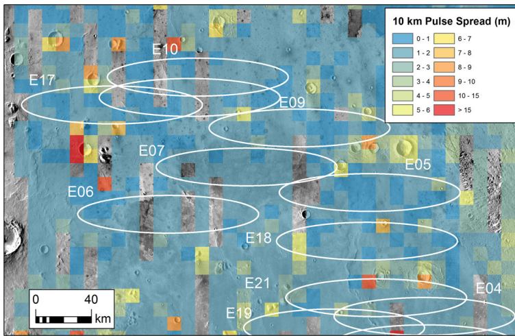
Fig. 20 Map of MOLA pulse spread (slope corrected from Neumann et al. 2003), which is a measure of the RMS relief within the ~75 m diameter laser spot, of the InSight landing sites. Note exceptionally low pulse spread of the smooth plains without large craters and the higher relief over large craters and monadnocks. Notice the similarity with the map of Allen deviation at roughly the same length scale in Fig. 19. Background is THEMIS daytime mosaic
