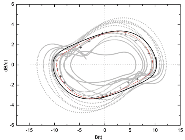
Fig. 5 Phase-space diagram for the toroidal proxy B_\phi(t) : The crosses correspond to local area averaged values found by dividing the data into 32 temporal intervals. The red dashed curve is a fit to the crosses. The continuous black curves correspond to a fit to all data points (not grouped in intervals). For the red curve we have that \mu = 0.1645 , \omega = 0.3523 , \xi = 0.0147 and \lambda = 0.0005 . Figure adapted from Passos and Lopes (2008a)
