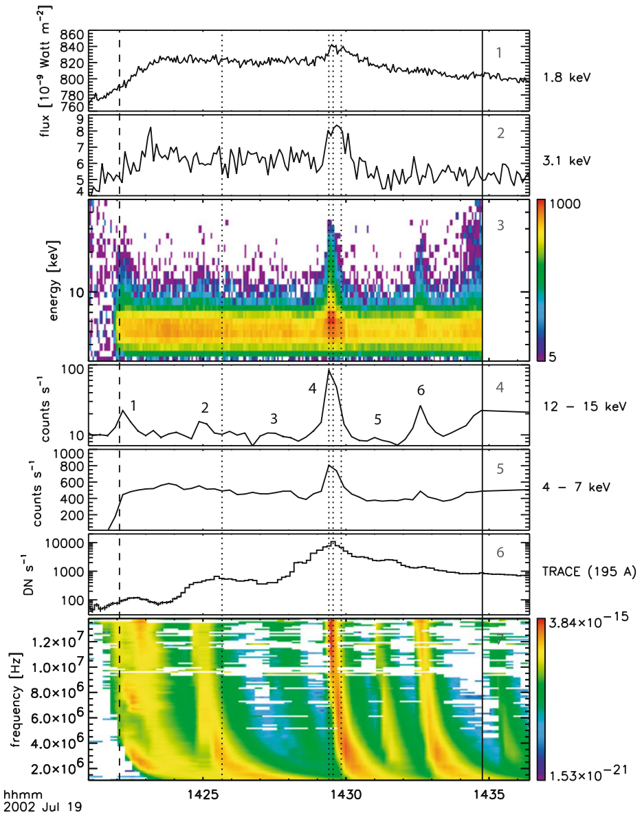
Fig. 11 The lightcurves and radio spectrograms of six RHESSI microflares from July 19, 2002 (Christe et al. 2008b). The top two panels show the GOES lightcurves in 1–8 Å (with a B8 background level) and 0.5–4 Å. The next three panels show the RHESSI spectrogram with night-time background removed and lightcurves in 12–15 keV (nonthermal) and 4–7 keV (thermal). The EUV lightcurve from TRACE and a radio spectrogram from WIND/WAVES are shown in the bottom two panels. The radio emission starts at around 14 MHz and drifts down to 2 MHz. It is well correlated with the RHESSI HXR lightcurve. Reproduced by permission of the AAS
