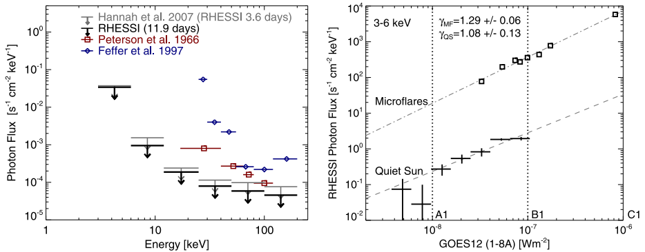
Fig. 12 Observations and upper limits of the quiet-Sun hard X-ray flux found with RHESSI . ( Left ) The RHESSI upper limits to the quiet Sun emission at 3–200 keV in comparison to previous observations (Hannah et al. 2010), including the first RHESSI quiet Sun limits (Hannah et al. 2007b). ( Right ) comparison of the 3–6 keV flux observed with RHESSI to the 1–8 Å GOES emission for the quiet Sun and offpointed microflares. The \gamma_{MF} and \gamma_{QS} indicate the index of power-law fits to the data, the dashed and dashed-dotted lines (Hannah et al. 2007b). Reproduced by permission of the AAS
