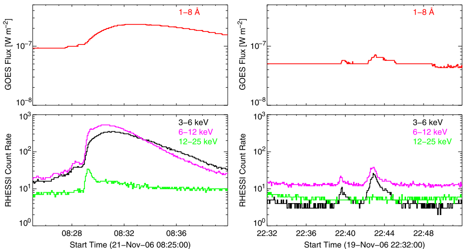
Fig. 6 The GOES 1–8 Å lightcurve (top panels) and RHESSI lightcurves for some example microflares. (Left) A single B-class microflare (B1 with pre-flare background subtracted) which shows the classic flare time profile: impulsive at higher energies with a slower rise and more gradual fall at lower energies. This event also shows some pre-flare emission. (Right) Two A-class events (A1 and A3, background-subtracted) both of which have no emission above 12 keV observed by RHESSI ; their nonthermal emission hidden by the background. Note that the background level in these microflares is predominantly solar for GOES , but terrestrial and instrumental in origin for RHESSI
