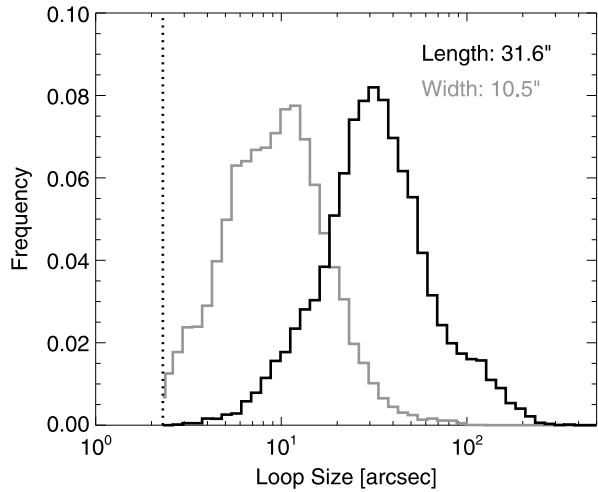
Fig. 9 Loop arc length and width distributions for 18,656 microflares imaged by RHESSI indicating that they are predominantly elongated structures (Hannah et al. 2008a). Thus microflares are not necessarily spatially small. Reproduced by permission of the AAS
