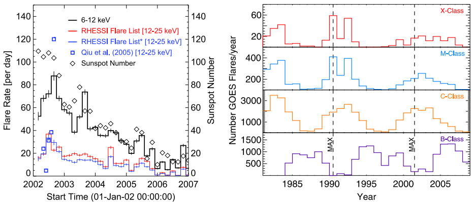
Fig. 5 (Left) Occurrence rate of RHESSI microflares (<C1 events) (Christe et al. 2008a), showing a clear decline over the waning years of Cycle 23. Reproduced by permission of the AAS. (Right) The number of GOES flares per year per flare class for X-class (top) through M, C to B-class (bottom). The microflares seem to be anti-correlated with the larger flares, which would be expected from the increased background during times of high activity. Note that B-class flare data was only available from 1984 (data from Milligan 2009)
