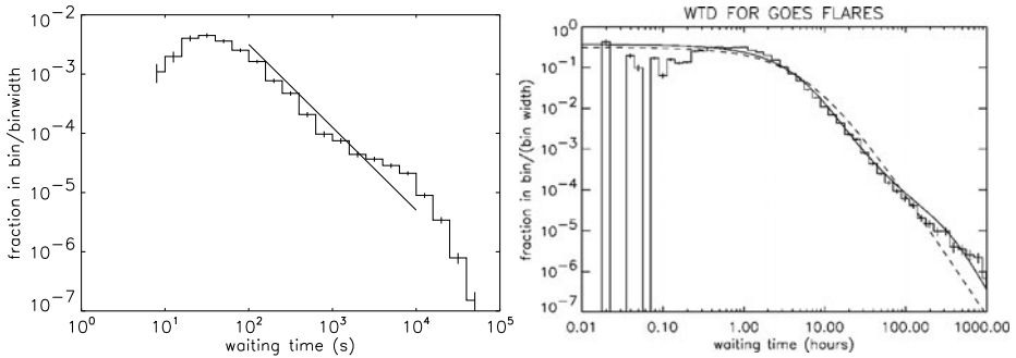
Fig. 16 Waiting-time distributions for different sets of X-ray flares. Left: ICE/ISEE-3 study of 6919 flares > 30 keV (Wheatland et al. 1998), the overplotted solid line is a power-law fit. Right: 32,563 GOES flares above C-class (Wheatland 2000), the overplotted lines indicate a model for a time-dependent Poisson process ( solid ) and independent events with an exponential distribution of rates ( dashed ). Reproduced by permission of the AAS
