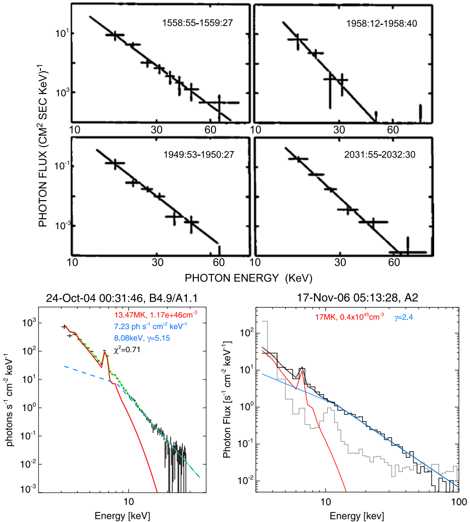
Fig. 7 (Top four panels) the first HXR microflare spectra from a balloon-borne instrument (Lin et al. 1984), and (bottom two panels) spectra from RHESSI showing a typical microflare (Hannah et al. 2008a) (left) and one with a particularly hard spectrum (right) (Hannah et al. 2008b). The red and blue lines are the thermal and nonthermal components of the model, respectively. In the RHESSI spectra, the upper limit of the nonthermal component is hidden by the instrumental background (the large errors bars in the bottom-left spectrum and the grey histogram in the bottom-right spectrum). Reproduced by permission of the AAS
