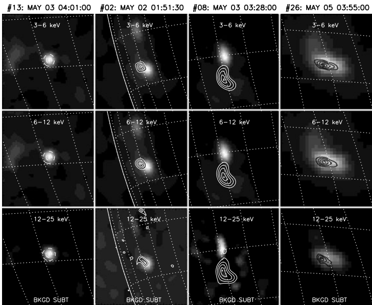
Fig. 10 Four microflares (one per column) imaged in different HXR energy bands (increasing from top row to bottom) with RHESSI (contours), overplotted on NoRH 17 GHz images (Kundu et al. 2006). The bottom microwave image is background-subtracted. Similar-sized footpoints and loop structures are seen in both HXRs and microwaves
