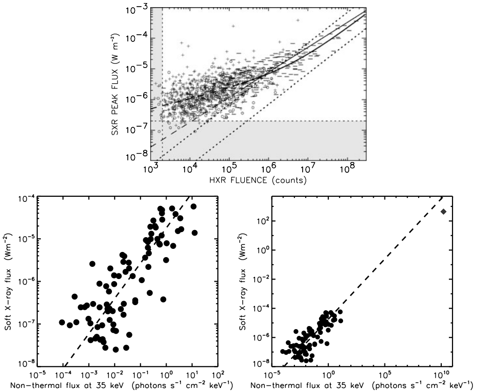
Fig. 23 Comparisons of thermal and nonthermal fluxes for ordinary flares. Upper : background-subtracted SXR peak flux from GOES vs. HXR fluence from HXRBS (Veronig et al. 2002b). The solid lines show various functional fits, the dashed lines show proportionality, with extension to smaller fluence, and the grey areas indicate regions below instrumental threshold. The different plot symbols indicate the time difference between SXR and HXR peaks. Lower : a representative sample of RHESSI flares (Battaglia et al. 2005), plus the same sample but including the enormous stellar flare observed by Osten et al. (2007) (the red point ). Again, the dashed line shows proportionality
