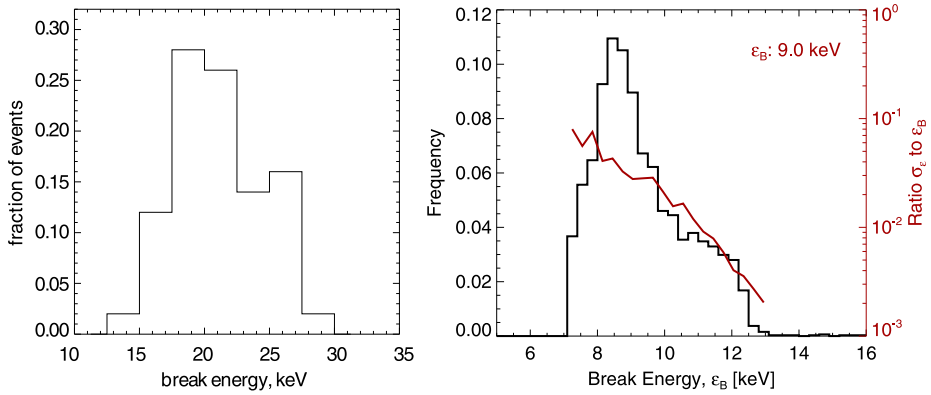
Fig. 19 Two examples of low-energy break energy distributions from fitting RHESSI photon flare spectra, ( left ) for 55 large occulted flares (Krucker and Lin 2008) and ( right ) 4236 microflares (Hannah et al. 2008a), the dark red line indicating the error ratio. Reproduced by permission of the AAS
