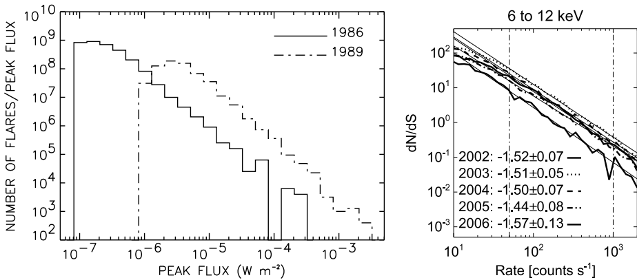
Fig. 14 Comparisons of occurrence distributions with phase in the solar cycle. ( Left ) Veronig et al. (2002a) using GOES 1–8 Å data from solar minimum (1986) to maximum (1989); ( right ) Christe et al. (2008a) using RHESSI microflare data from leaving solar maximum (2002) through to approaching solar minimum (2006). Reproduced by permission of the AAS
