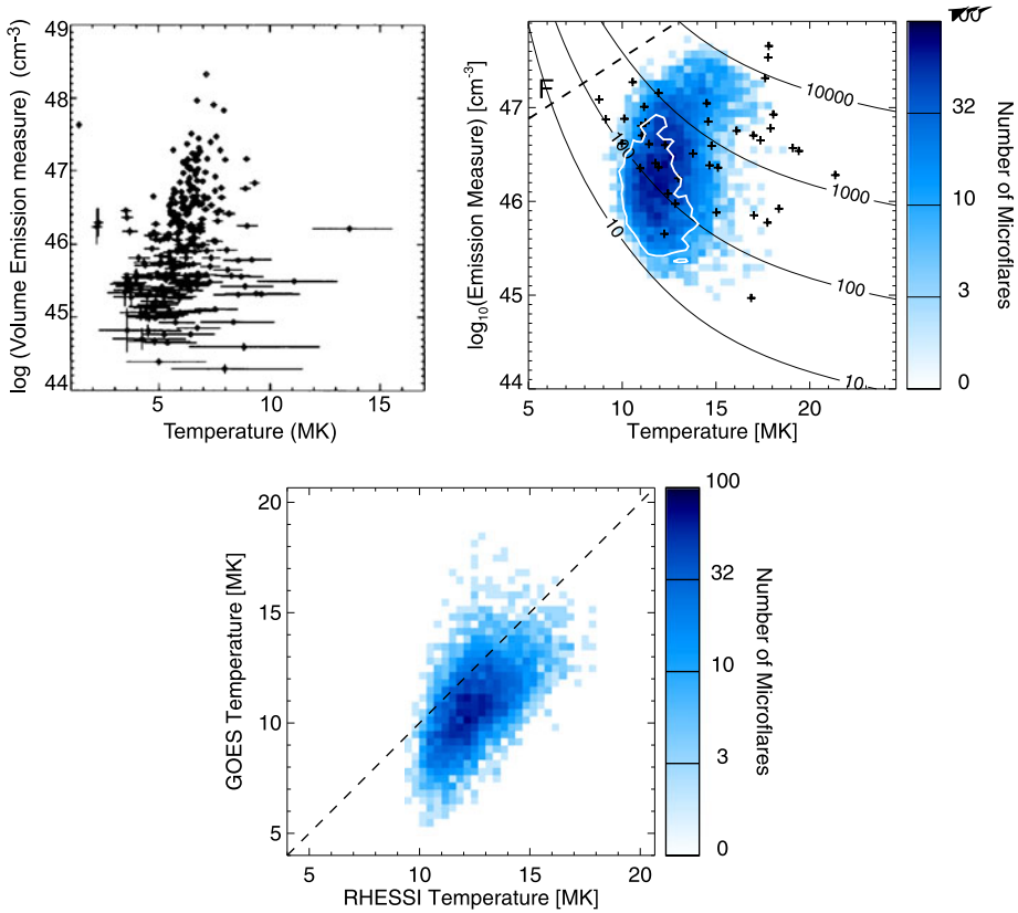
Fig. 21 Thermal parameter surveys of microflares. ( Top left ) 291 Yohkoh/SXT microflares (Shimizu 1995) (his “active region transient brightenings”). Reproduced by permission of the PASJ. ( Top right ) 9161 RHESSI microflares (Hannah et al. 2008a). The numbered solid lines show expected 4–8 keV RHESSI counting-rate levels as a function of model T and EM, the white contour shows the events with GOES T < 10 MK from the bottom panel and the dashed line (F) the relationship between emission measure and temperature found by (Feldman et al. 1996); see Fig. 22. Note that neither of these studies individually confirms this correlation, and that the two data sets are almost disjoint. ( Bottom ) The microflare temperature derived using both RHESSI and GOES for 6740 microflares (Hannah et al. 2008a). Reproduced by permission of the AAS
