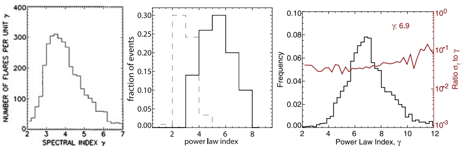
Fig. 17 Distributions of HXR power-law index \gamma for Left : 6919 large flares observed above 30 keV with ICE/ISEE-3 (Bromund et al. 1995); middle : 55 large flares on the disk ( dashed grey ) and occulted ( solid black ) with RHESSI (Krucker and Lin 2008). Right : 9161 RHESSI microflares from the sample of Hannah et al. (2008a), the dark red line indicating the error ratio. Reproduced by permission of the AAS
