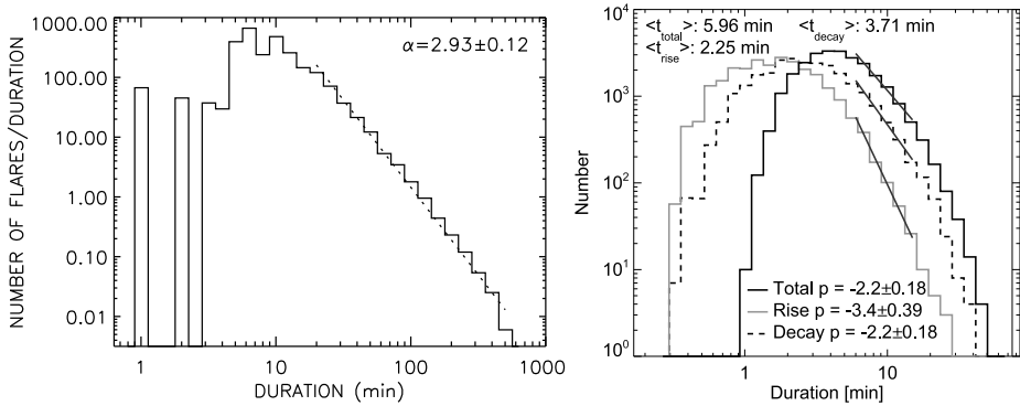
Fig. 15 Left : the distribution of the durations of flares GOES >B class (Veronig et al. 2002a); right : distribution of durations of microflares (Christe et al. 2008a), typically below GOES C class. Reproduced by permission of the AAS
