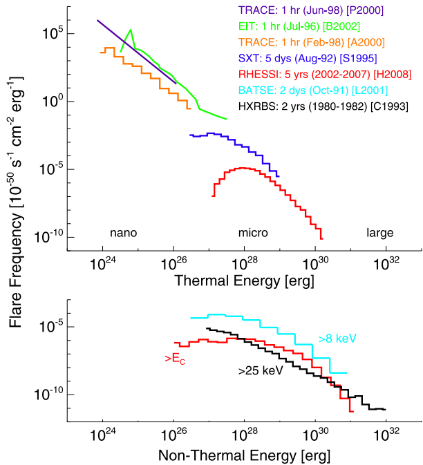
Fig. 2 The energy distributions for solar flares. The nonthermal energy distribution is shown for large flares > 25 keV observed with SMM /HXRBS (Crosby et al. 1993), microflares > 8 keV from CGRO /BATSE (Lin et al. 2001a) and microflares > E_C (above the low energy cutoff) from RHESSI (Hannah et al. 2008a). The thermal energy distribution is shown for microflares with RHESSI (Hannah et al. 2008a) and Yohkoh /SXT (Shimizu 1995) and EUV nanoflares with TRACE (Parnell and Jupp 2000; Aschwanden et al. 2000) and SOHO /EIT (Benz and Krucker 2002). This figure is deceptive as it is comparing energy distributions of different flare energy components, each involving different instrument and selection effects, and were obtained over different periods of different solar cycles
