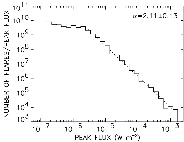
Fig. 1 Frequency distribution of the peak 1–8 Å SXR GOES flux of 49,409 flares between 1976 and 2000 (Veronig et al. 2002a). Note that this study did not include the A-class events ( <10^{-7} \text{ W m}^{-2} ). In addition, there was no attempt at background subtraction, so the resulting value of \alpha should be regarded as an upper limit (background predominantly affects smaller flares, artificially steepening the distribution)
