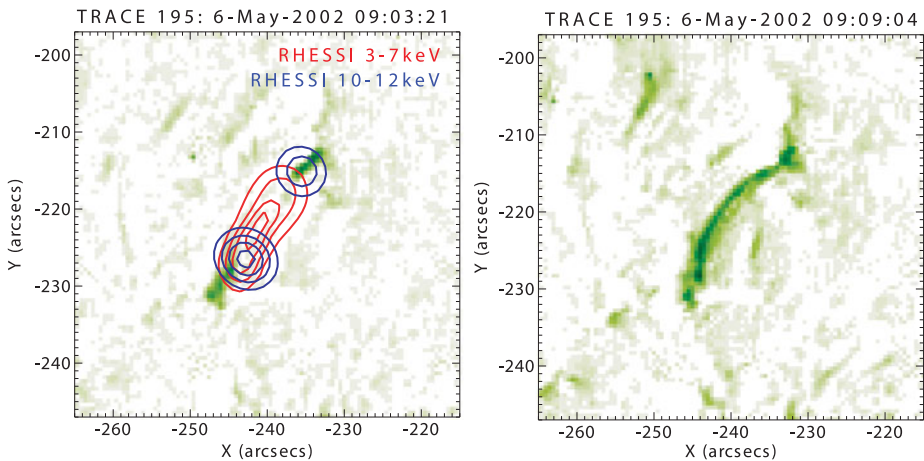
Fig. 8 Overlay of RHESSI thermal (red) and nonthermal (blue) contours on TRACE , showing the typical flare and microflare scenario of (left) footpoints depositing their energy to heat chromospheric material that expands upwards, filling the loops connecting them. (Right) this material then cools, emitting brightly in EUV. Updated version of figure from Krucker et al. (2002)
