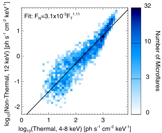
Fig. 24 Thermal/nonthermal correlation for 4236 RHESSI microflares (Hannah et al. 2008a). The nonthermal flux is the estimated 12 keV emission using the fitted nonthermal model. The thermal flux is found from fitting the X-ray visibilities over 4–8 keV. Note that the axes are inverted relative to those of Fig. 23, but that the line of proportionality is the same. Reproduced by permission of the AAS
