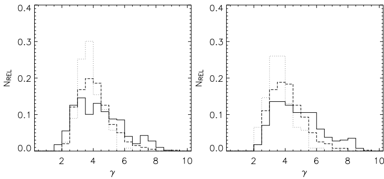
Fig. 18 The effect of albedo correction on the observed HXR power-law index, with histograms of \gamma ( left ) found from spectrum fitting and ( right ) then corrected for albedo (Kašparová et al. 2007). The different lines show the power-law fits made over different energy ranges: 398 flares with \gamma_0 ( solid ) 15–20 keV and \gamma_1 ( dashed ) 20–35 keV, and 123 flares with \gamma_2 ( dotted ) 35–50 keV
