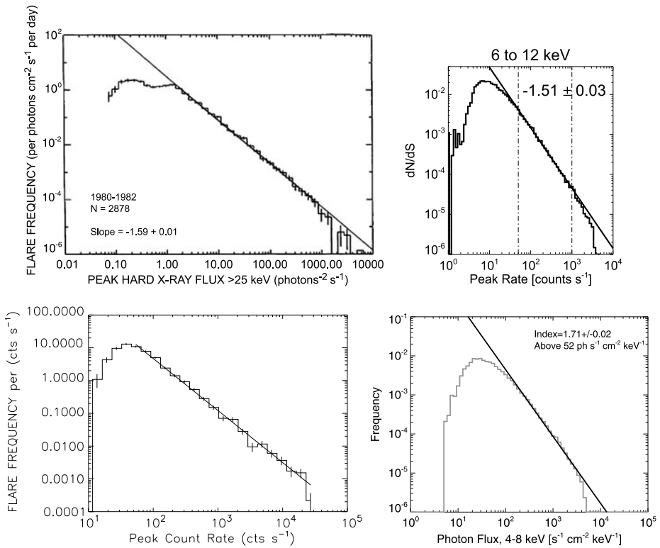
Fig. 13 Several of the flux distributions listed in Table 2 (Crosby et al. 1993, 1998; Christe et al. 2008a; Hannah et al. 2008a) (left to right, top to bottom). Another example (Veronig et al. 2002a) is shown in Fig. 1. Reproduced by permission of the AAS
