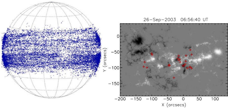
Fig. 4 (Left) The locations of 24,097 microflares observed with RHESSI between March 2002 and March 2007 (Christe et al. 2008a). All of the confirmed events could be associated with active regions. Reproduced by permission of the AAS. (Right) The locations of one day of RHESSI microflares from active region 10456 (Stoiser et al. 2007). Of 53 events found, 24 could be imaged. The centroid positions (3–6 keV) are indicated by crosses and overlotted on the MDI (Michelson Doppler Imager of SOHO ) magnetogram
