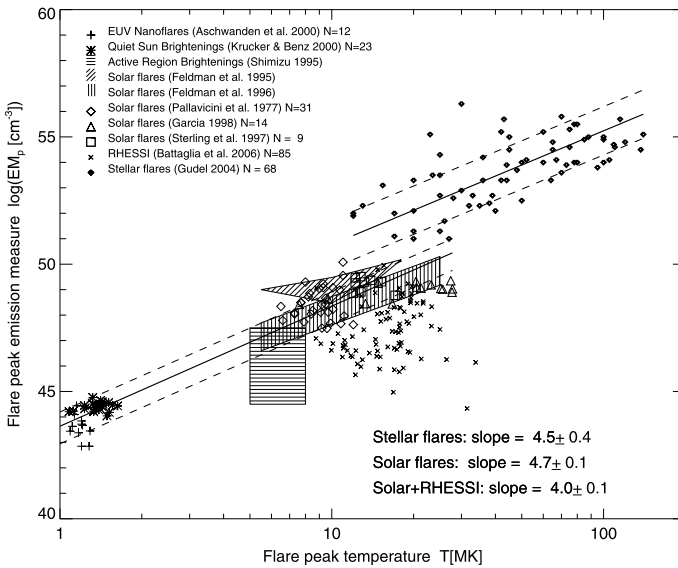
Fig. 22 Thermal fits from various surveys showing the correlation of emission measure (log scale) with temperature of solar flare observations compared with observations of stellar flares and with quiet-Sun brightenings, from the sources shown (Aschwanden et al. 2008). Reproduced by permission of the AAS
