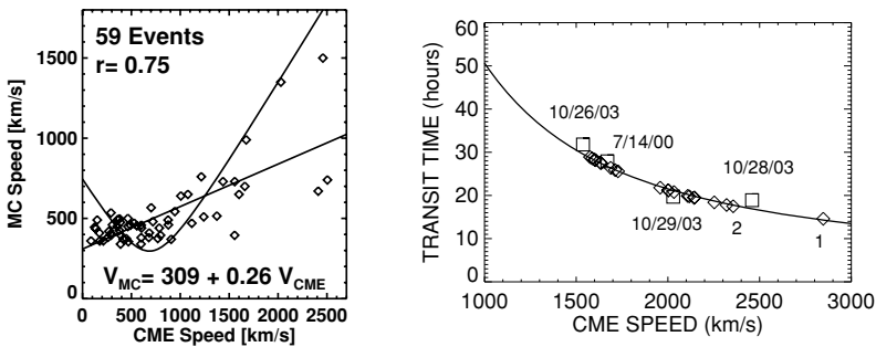
Figure 8. (left) CME and MC speeds for the 59 CME-MC pairs. The straight line is Lindsay et al. (1999) formula. The parabolic curve is from Gopalswamy et al. (2001b). (right) the empirical shock arrival model for (solid curve) with some very fast events (diamonds) including the Carrington events of 1859 September 1 (marked 1) and August 4, 1972 (marked 2). The squares are actual measurements of CME speeds from SOHO and the observed shock transit times.
