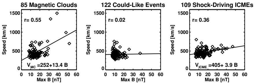
Figure 5. Correlation between the speed and magnetic field strength of MCs (left), cloud-like events (middle) and shock-driving ICMEs (right). The correlation coefficient ( r ) is marked in each case.
