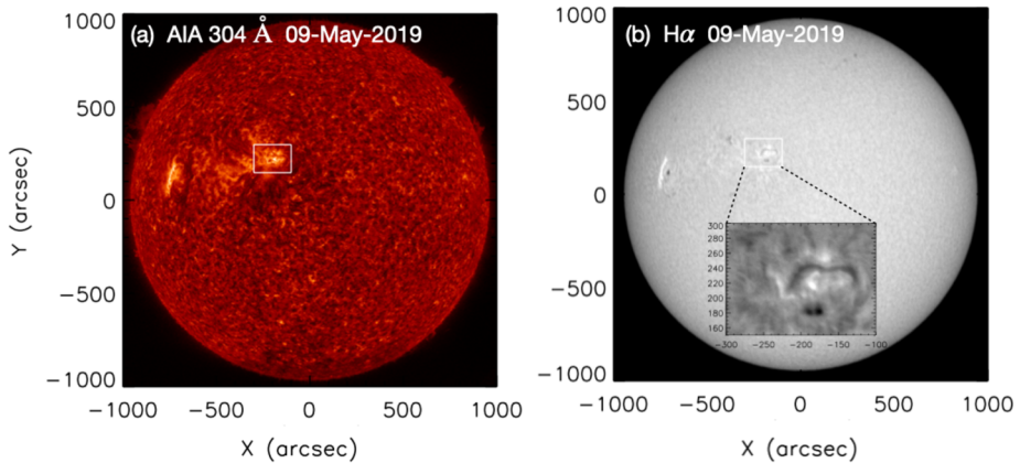
Figure 1 Full-disk images showing AR 12740 ( white box ) in: (a) AIA 304 Å band and (b) in GONG Learmonth H\alpha image on 9 May 2019 at 05:39 UT including a zoom on the filament. The white box in panel b covers the FOV of Figures 5 and 6.
