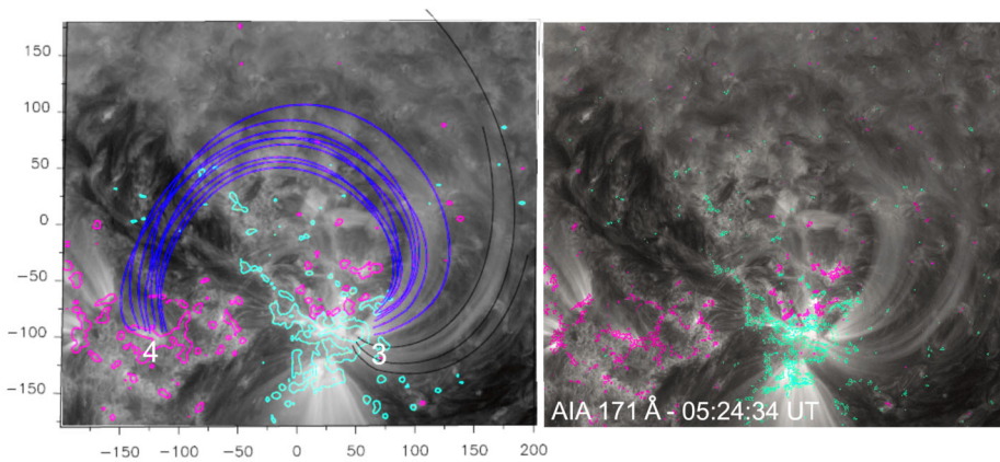
Figure 12 Left panel: Magnetic field model of the large-scale coronal loops connecting the chain of small negative polarities labelled as 3 to the disperse positive following AR polarity 4 (see Figure 2). A set of computed field lines in blue solid traces is overlaid on the AIA 171 image at 05:24:34 UT, together with HMI magnetic field contours ( \pm 100, 500 G, positive (negative) shown in magenta (blue) colour). The three black field lines connect to northern positive quiet-Sun regions out of the AR (compare to Figure 16). The axes in this panel are in Mm, with the origin set at the AR centre. Right panel: The same AIA image shown as background in the left panel for comparison. The image is shown in logarithmic direct intensity and we have added HMI isocontours of similar values to those in the left panel as a reference. The images are shown in grey scale to facilitate the visualisation of computed field lines and magnetic field contours in this figure and the following two.
