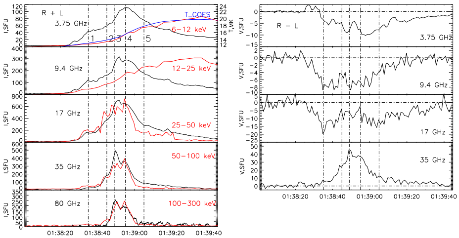
Figure 1 Light curves of X-ray (RHESSI, red) and microwave fluxes (NoRP, black) in intensity ( R + L , left) and in polarization ( R - L , right). Plasma temperature profiles calculated from the GOES data are shown in the top left panel. The RHESSI data are presented in arbitrary units.
