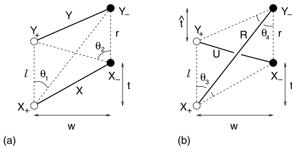
Figure 2 The geometry for quantifying a “simple zippette”, a typical single reconnection event in the zipper phase of a sheared coronal arcade. (a) The initial configuration ( XY ), in which sources X_+ and X_- are connected by one flux tube ( X ), and Y_+ and Y_- are joined by a second tube ( Y ). (b) The final configuration ( UR ), in which the initial flux tubes have reconnected to form a flux rope ( R ) connecting X_+ to Y_- . This lies above a second underlying flux loop ( U ), which connects Y_+ to X_- . Interior angles ( \theta_j ) are indicated for both configurations.
