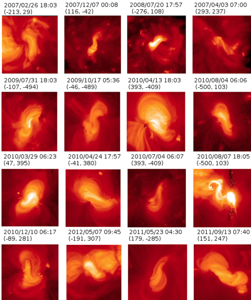
Figure 1 A collection of sigmoid cutout images from Hinode/XRT in the Ti/poly filter. Some of the sigmoids are S-shaped and some have an inverted-S shape. These sigmoids vary in size and the field of view of all images is the same -256'' \times 256'' . The time and center of the field of view in arcsec are given above the images.
