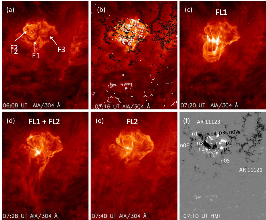
Figure 7 (a) Filaments F1, F2, and F3, embedded in AR 11123, observed in absorption on 11 November 2010 at 06:08 UT. (b)–(e) Different stages of the eruption of filament F1, low-energy event preceding (or precursor to) FL1 and flare (FL1 and FL2) brightenings. The upper-chromosphere images are observed with AIA at 304 Å. Isocontours ( \pm 50 , \pm 100 G, white (black) continuous lines for positive (negative) field values) of the HMI image shown in panel (f) have been added as a guide in panel (b). (f) HMI line-of-sight magnetic field covering the same field of view as the AIA images. The polarities involved in the studied events are labelled. For clarity, these labels are placed at the side of the polarities in AR 11123. A detailed description of the evolution illustrated in these images is provided in Section 3.4. The size of each panel is 240'' (300'') in the horizontal (vertical) direction. The centre of each panel in heliographic coordinates is located at [-165'', -485''] ; Sun's centre is at [0'', 0''] .
