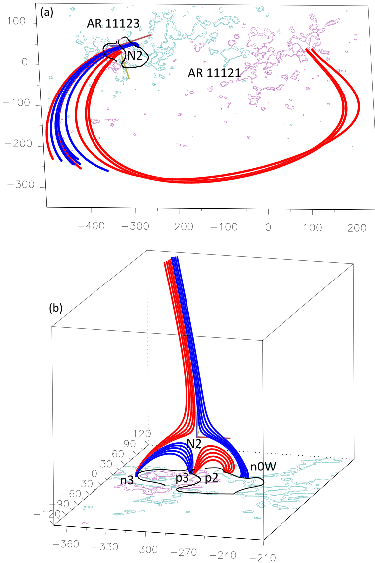
Figure 11 Coronal magnetic-field model in the close vicinity of magnetic null point N2. (a) The set of N2 fan field lines following the upper spine connected to AR 11121 are shown in the observer’s point of view. (b) Close-up view showing two sets of field lines representing the pre-reconnected lines (in blue colour) and reconnected lines (in red colour), as inferred from the observed evolution described in Section 3.4 and our interpretation in Section 5.3. In both panels the black continuous lines correspond to the photospheric trace of QSLs (see Section 5). All axes are in Mm and the isocontours of the field correspond to \pm 50 , \pm 100 G in continuous magenta (blue) style for the positive (negative) values.
