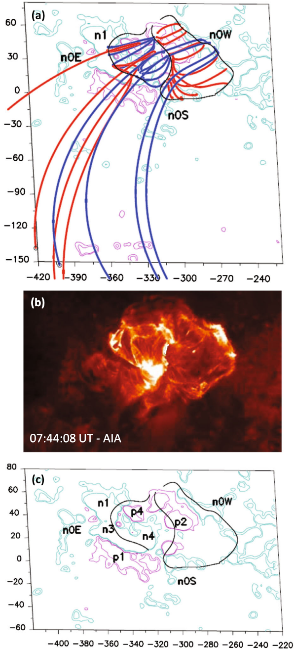
Figure 14 Comparison of QSLs and ribbons of flare FL2.
