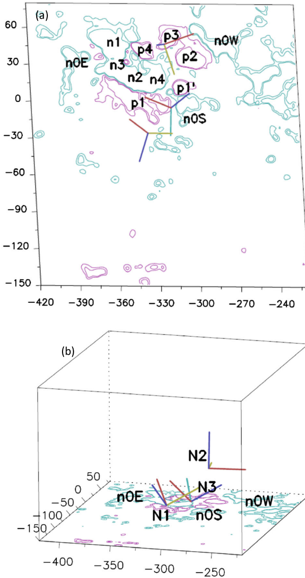
Figure 9 Location of the three null points associated with the magnetic configuration of AR 11123 on 11 November 2010. (a) Observer's point of view showing the three null points. For reference, we have numbered the polarities as in Figure 4. (b) Perspective view selected to illustrate the height of the nulls above the photosphere, which are numbered N1, N2, and N3. Some of the polarities are labelled as in Figure 4. In both panels, all axes are in Mm and the isocontours of the field correspond to \pm 50 , \pm 100 G in continuous magenta (blue) style for the positive (negative) values. The three segments at the locations of the nulls correspond to the direction of the three eigenvectors of the Jacobian matrix. The colours of these segments indicate the magnitude of the corresponding eigenvalue, red (yellow) corresponds to the largest (lowest) positive eigenvalue in the fan plane and blue to the spine eigenvalue for a positive null point (N1 and N2 in our study). In the case of a negative null (N3 in our study), light blue (dark blue) corresponds to the largest (lowest) negative eigenvalue in the fan plane and red to the spine eigenvalue. From now on, the field of view of each figure will be chosen according to the magnetic structures that we want to show. As a guide, we will label in each figure some of the polarities as in Figure 4.
