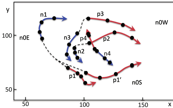
Figure 3 Summary of the evolution of the polarities during the emergence of AR 11123. The polarities are labelled as in Figure 2. Magenta (blue) colour is used for the path of positive (negative) polarities. The heads of the arrows indicate the polarity positions at 12:00 UT on 11 November 2010. Neighbour dots and corresponding arrow head are separated backwards by 12 hours. An extension of the arrow head indicates that a polarity was present at \approx 00:00 UT on 10 November 2010 (initial time of magnetic-evolution.mpg ). Dashed lines link the polarities belonging to the same bipole, when they appear separated.
