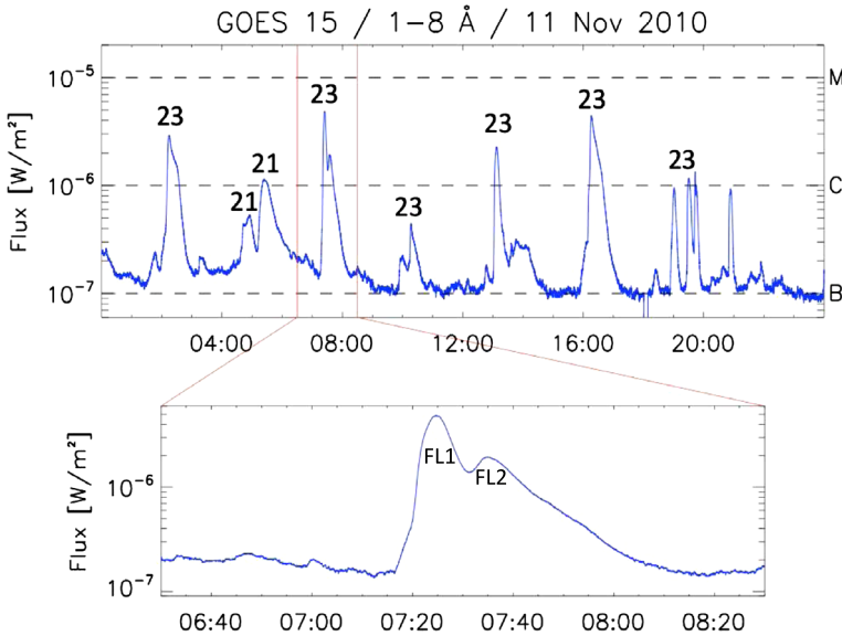
Figure 6 Soft X-ray flux as recorded by GOES in the 1–8 Å energy band. The top curve shows the flares on 11 November 2010, while the bottom curve is an enlargement at the time of the events described in Section 3.4. The numbers above the different flare maxima in the top curve correspond to the AR where they occur (21 stands for AR 11121 and 23 for AR 11123). The labels in the bottom enlargement indicate the events that we discuss in detail in Section 3.4.
