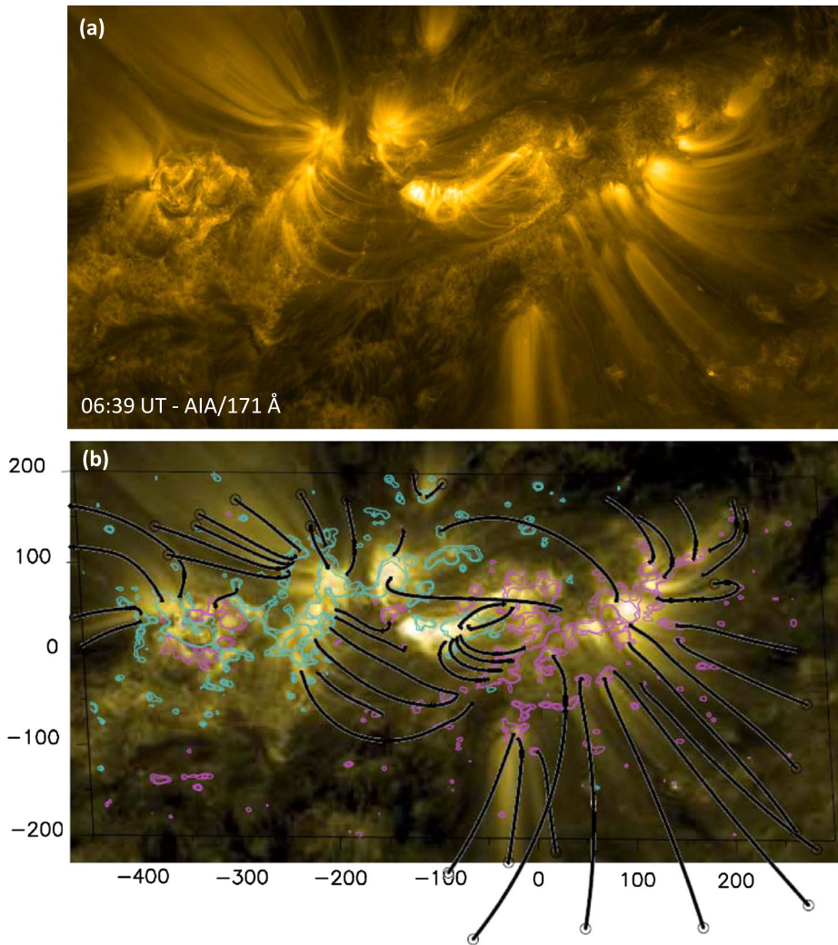
Figure 8 Coronal magnetic-field model of the AR complex. (a) AIA 171 Å image. The size of this panel is 690'' ( 390'' ) in the horizontal (vertical) direction. Its centre in heliographic coordinates is located at [-50'', -440''] ; Sun's centre is at [0'', 0''] . (b) Field lines (black continuous lines), computed from the LFFF model, that best fit AIA loops for a value of \alpha = 3.1 \times 10^{-3} \text{ Mm}^{-1} . The field lines ending in an open circle reach the 3D box selected for the figure (only its base is shown). The axes in this panel are in Mm and the isocontours of the field correspond to \pm 50 , \pm 100 G in continuous magenta (blue) style for the positive (negative) values. These are overlaid on the AIA image shown in (a).
