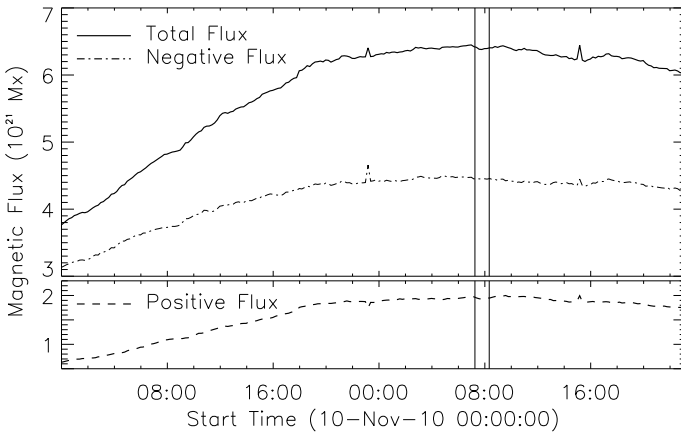
Figure 5 Magnetic-flux evolution in AR 11123. The flux is computed for the same field of view shown in Figure 4(a) within the green rectangle. The existence of a negative background is evident in the figure, as the negative magnetic flux is much higher than the positive one. The magnetic flux emerging in bipoles should be roughly balanced; however, this is not the case for AR 11123, because it emerges within the (already decaying) following negative polarity of AR 11121. The two vertical lines indicate the start and end times of the series of events discussed in detail in Section 3.4.
