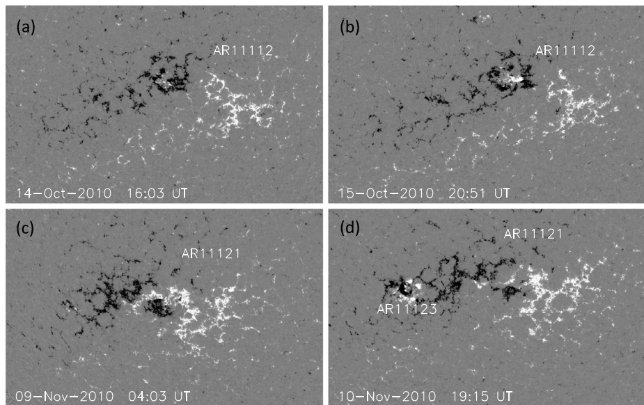
Figure 1 Large magnetic-field complex in the southern hemisphere during (a, b) October and (c, d) November 2010. The magnetograms show some of the bipole emergences within a long-living AR. AR 11123 was born in the negative-field environment of the following polarity of AR 11121 during the November rotation (panel (d)). White (black) regions are positive (negative) line-of-sight magnetic polarities. The magnetic-field values have been saturated above (below) 500 G ( -500 G). The size of each panel is 800'' in the E–W (East–West) and 500'' in the N–S (North–South) direction. The centre of each panel in heliographic coordinates changes from one solar rotation to the other, being located at [-80'', -455''] in the first panel; Sun’s centre is at [0'', 0''] .
