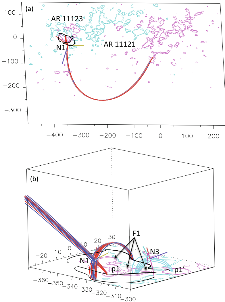
Figure 10 Coronal magnetic-field model in the close vicinity of magnetic null points N1 and N3. (a) Large-scale connection of the spine of null N1. The set of N1 fan field lines, following the upper spine, connected to AR 11121 are shown in the observer's point of view. (b) Close-up view showing sets of field lines drawn from the close neighbourhood of null points N1 and N3. In the case of N1, field lines represent pre-reconnected (in blue colour) and reconnected ones (in red colour), as inferred from the observed evolution described in Section 3.4 and the interpretation in Section 5.2. For N3, the spine is drawn in pink and a set of fan field lines in light blue. The arrows in panel (b) point to the location of filament F1 along the PIL between n_2 – n_4 and p_1 – p_1' . In both panels, the black continuous lines correspond to the photospheric trace of QSLs (see Section 5). All axes are in Mm and the isocontours of the field correspond to \pm 50 , \pm 100 G in continuous magenta (blue) style for the positive (negative) values.
