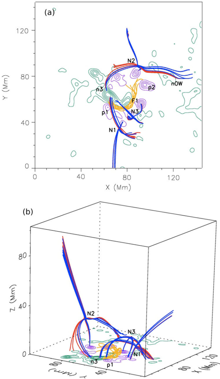
Figure 12 Magnetic-field model of AR 11123 in the vicinity of the null points in the NLFFF approximation. (a) Point of view in which the region is located at central-meridian passage. Blue and red field lines represent the magnetic domains before and after the magnetic reconnection, respectively, following the convention in Figures 10 and 11. Orange field lines depict the magnetic-field structure of filament F1 which lies along the PIL between n2-n4 and p1-p1' (see Figures 7 and 10(b)). (b) Point of view selected to better show the 3D structure of the field lines. In both panels the magnetic-field contours correspond to the photospheric vertical-field component in the range [-1600, 1600] G, which is divided into 12 levels with a difference of 291 G between two adjacent levels.
