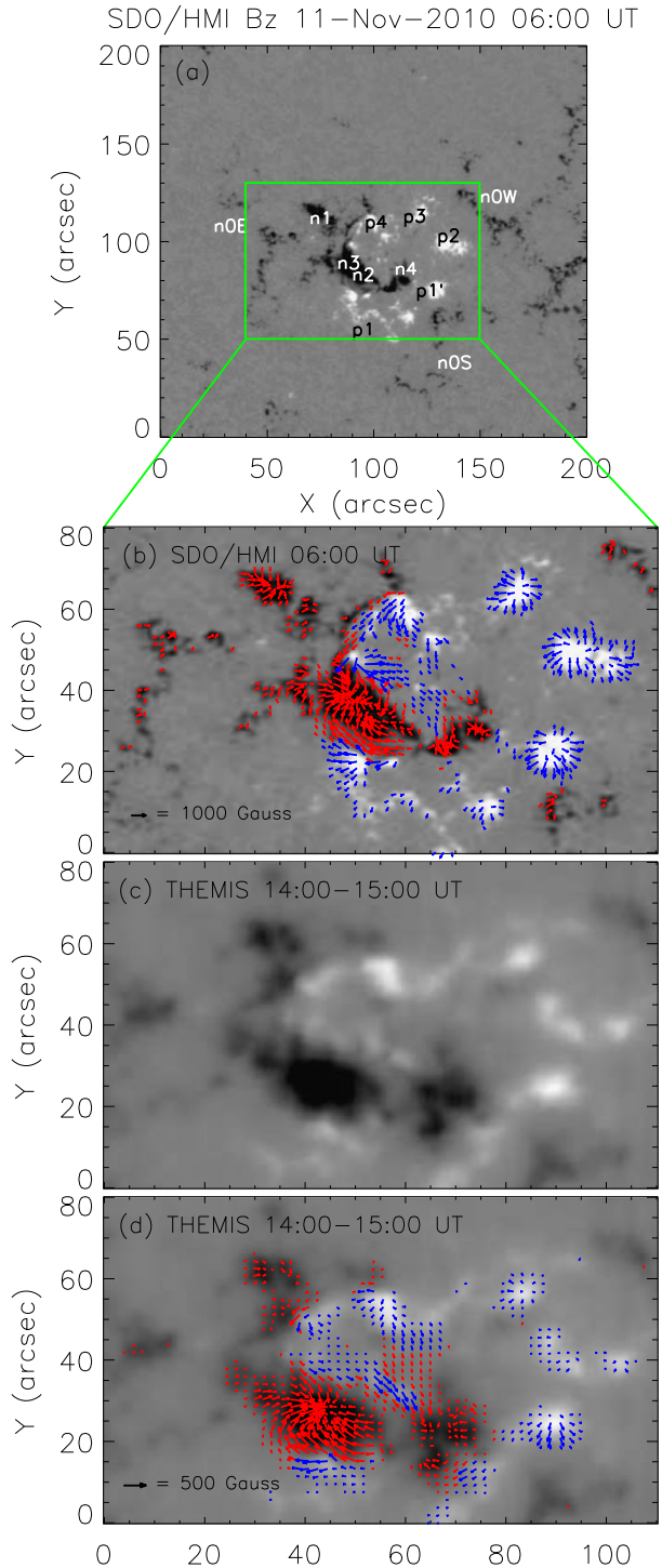
Figure 4 (a) and (c) Vertical [ B_z magnetic-field component] observed with HMI at 06:00 UT and with THEMIS between 14:00–15:00 UT, respectively. (b) and (d) Vertical and horizontal components observed with both instruments. White (black) regions correspond to positive (negative) polarities. The vertical-field values have been saturated above (below) 1000 G (– 1000 G) for HMI and above (below) 500 G (– 500 G) for THEMIS. The blue (red) arrows indicate the direction of the horizontal-field component for the positive (negative) vertical-field regions. The arrow density is uniform above (below) a vertical-field value of 250 G (– 250 G) for HMI and 40 G (– 40 G) for THEMIS. The length of the arrows is proportional to the horizontal-field intensity. Labels on the polarities in panel (a) indicate the different emerging bipoles (see Section 3.2).
