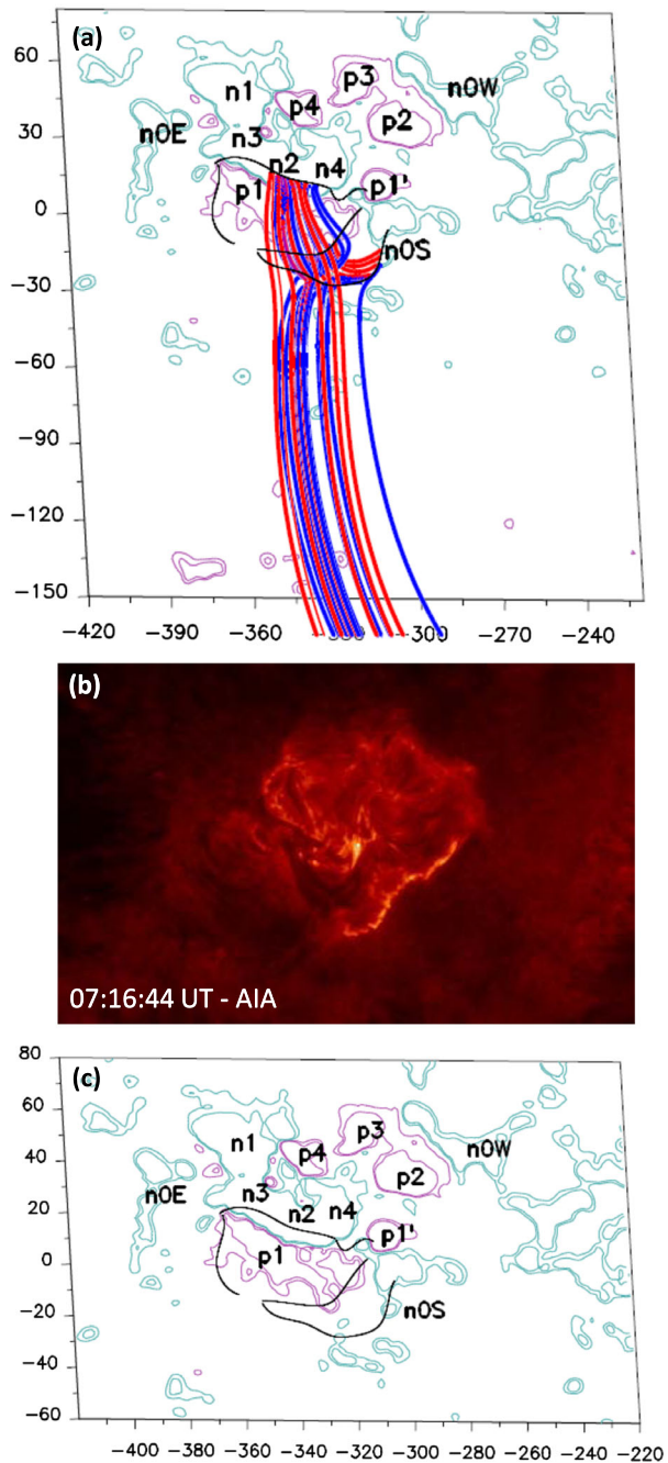
Figure 13 Comparison of QSLs and brightenings of the low-energy precursor to flare FL1. (a) Photospheric trace of QSLs in AR 11123 computed on the polarities associated with null N1 and field lines originating in the QSLs. Blue and red field lines indicate pre-reconnected and reconnected loops. The field lines that leave the drawn box correspond to large-scale loops connecting to a positive polarity at the Southeast in AR 11121 (see Figure 10(a)). (b) An AIA 304 Å image in which an elongated brightening along polarity n0S and other minor ones on polarities n2 and n4 are present. The size of this panel is 240'' (150'') in the horizontal (vertical) direction. Its centre is located at [-175'', -430''] in heliographic coordinates; Sun's centre is at [0'', 0''] . (c) Photospheric QSL traces and magnetogram. This panel is a section of panel (a) and the field of view is the same as in panel (b). There is a close resemblance between the shape of the southernmost QSL and a section of the AIA brightening to the South of n0S, while the emission on n2 and n4 lies along the northernmost QSL. The shape of the western extension of the elongated band follows the shape of a section of the QSLs in Figure 14, see Section 5.2 for a plausible explanation. In panels (a) and (c), all axes are in Mm and the isocontours of the field correspond to \pm 50, \pm 100 G in continuous magenta (blue) style for the positive (negative) values.
