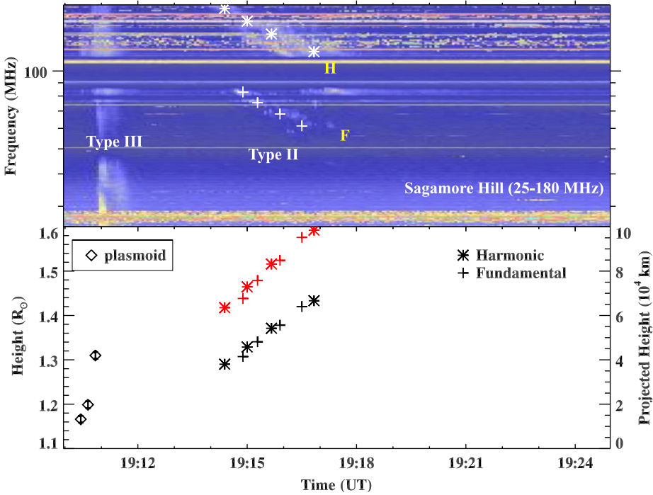
Figure 7 Top: The dynamic radio spectrum in 25 – 180 MHz observed at Sagamore Hill station on 16 October 2010, showing type III and type II radio bursts during the flare. Bottom: The source heights of type II burst inferred from the fundamental band (+) and harmonic band (*) using Newkirk 1-fold (lower) and 2-fold (upper, red) density models, respectively. The scale for the projected height (y-axis) of the plasmoid (diamond) is given on the right side (note the different units).
