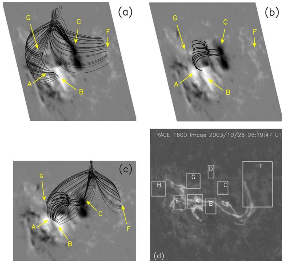
Figure 4. Extrapolated magnetic field lines using the longitudinal magnetic field observed by THEMIS at 08:55:52 UT for the active region NOAA 10486. The THEMIS magnetogram has been inserted in a large MDI map obtained at 07:15:03 UT ( 390'' \times 390'' ) to take advantage of high spatial resolution of THEMIS. The extrapolation was performed under the assumption of a current-free field. (a) A bird's-eye view of the high-altitude null, (b) A bird's-eye view of the low-altitude null, (c) A radial ( top ) view of both nulls, and (d) TRACE 1600 Å image at 06:19:47 UT. The boxes labeled 'A'–'H' indicate the eight regions we discuss in this paper.
