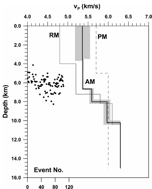
Fig. 4. P -wave velocity cross-sections: RM is the upper part of the model of Rigo et al. (1996) ; AM is the local model found for the area of Aigion; PM is the upper part of the model used for earthquake location in western Greece by the PATNET. The shaded zone gives the standard deviations of the AM model obtained by delete-one jackknifing. The group of dots represents the depth distribution of the 88 hypocentres (the corresponding horizontal coordinates represent the sequential numbers of earthquakes).
