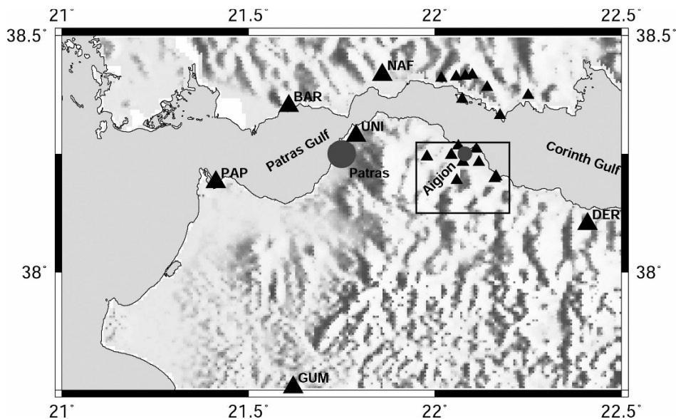
Fig. 1. Broader view of a part of the Gulf of Corinth with the area of interest delimited by the square. Positions of the CRL stations are shown as triangles, and the position of the nearest PATNET stations, up to a distance of 70 km from the town of Aigion (circle), are shown as larger triangles.
