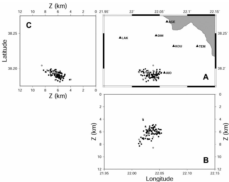
Fig. 2. Sequence of earthquakes that occurred in the region of Aigion in 2001: A) CRLNET stations used in this study (triangles) and the epicentres of the 104 stronger events (circles). The selected 88 events are shown as black circles. B) Projection of the hypocentres onto the longitude-depth plane. C) Projection of the hypocentres onto the latitude-depth plane.
