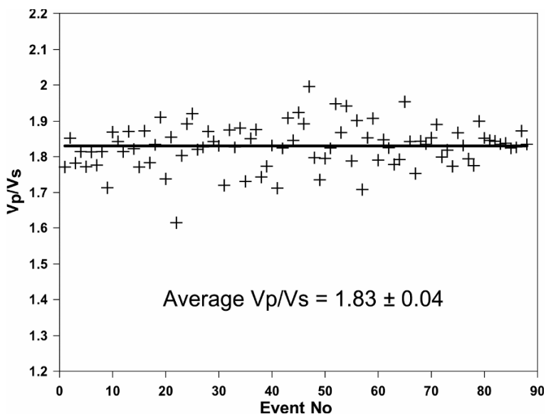
Fig. 3. The v_P/v_S ratios for the individual earthquakes obtained by the Wadati method.
