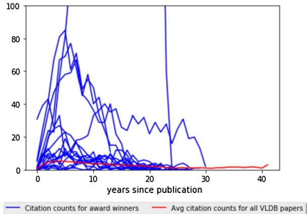
Fig. 2 VLDB test of time award winners versus all VLDB papers. One paper has so many citations that including its peak would make the bottom third of the graph unreadable
