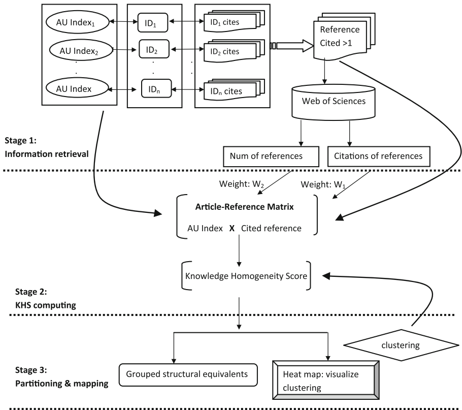
Fig. 3 Flow chart for author identification
