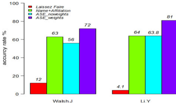
Fig. 7 Comparison of name disambiguation methods (as discussed earlier, the third category of extant disambiguation methods require comprehensive data collection and coding, and involve lots of subjective decisions when dealing with missing data. We could not replicate them in these two cases and thus have not included these more elaborate methods for accuracy rates comparison. In terms of time spent, it is reasonable to believe they are more time consuming than the ASE or name + affiliation methods)
