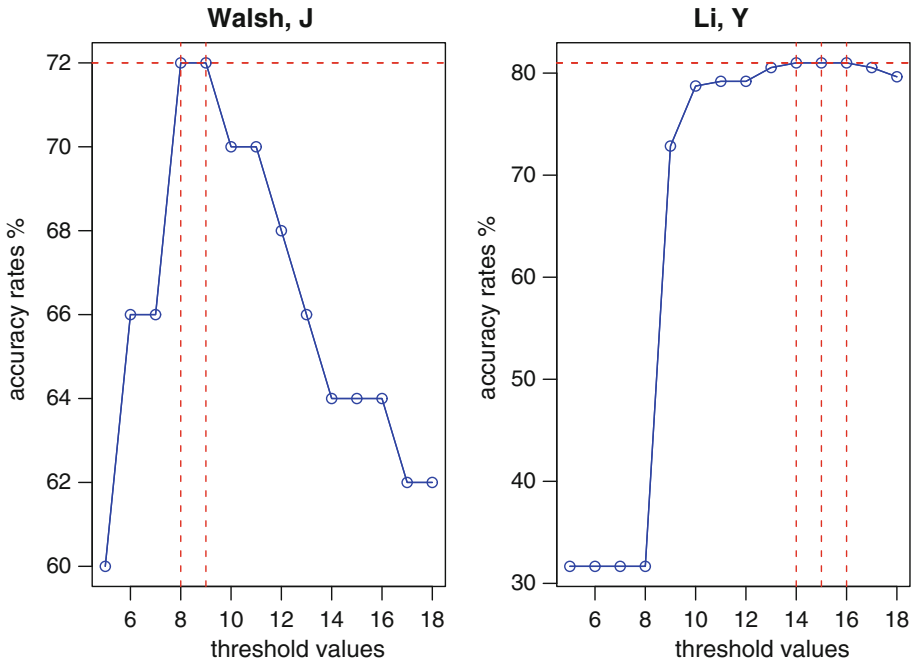
Fig. 8 Sensitivity tests on knowledge homogeneity thresholds
