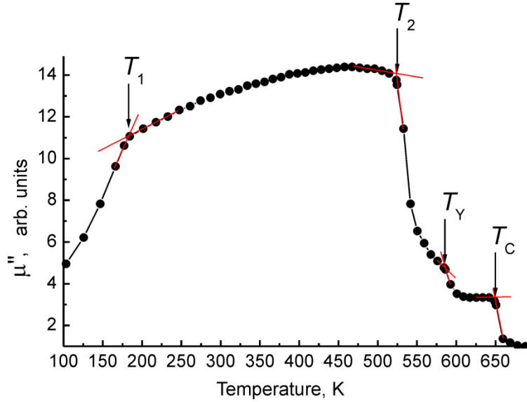
Fig. 4. Temperature dependence of initial magnetic permeability of Co 2 Z hexaferrite: T_1 – temperature of EMC ↔ EMP transition, T_2 – temperature of EMP ↔ EMA transition, T_Y – Curie temperature of Y phase, T_C – Curie temperature of Z phase.
