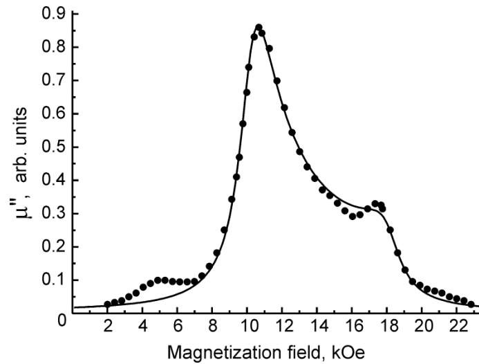
Fig. 5. Resonance curve of \text{Co}_2\text{Z} hexaferrite at the frequency of 38.32 GHz: the points stand for the experimental data, the solid line indicates the estimation for the following parameters of the material \gamma/2\pi = 2.84 GHz/kOe, H'_{a1} = -4.7 kOe, H_{a2} = -3 kOe, H_{a3} = H_\Phi = 0 kOe, M_S = 270 Gs, \alpha = 0.07 .
