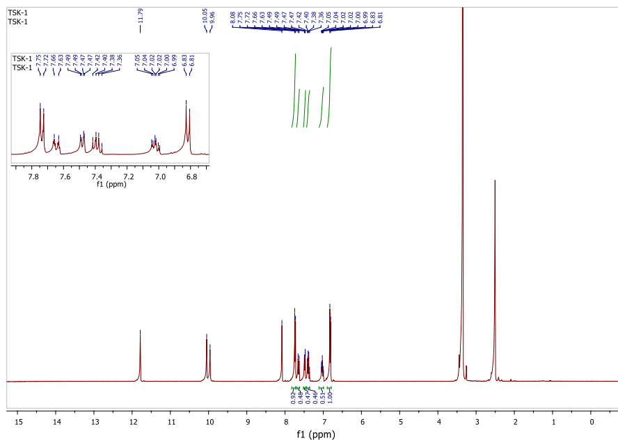
Fig. 2 ^1\text{H} NMR spectrum of compound IV
