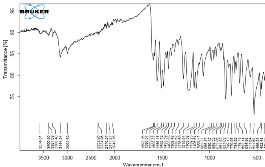
Fig. 1 IR spectrum of compound IV
