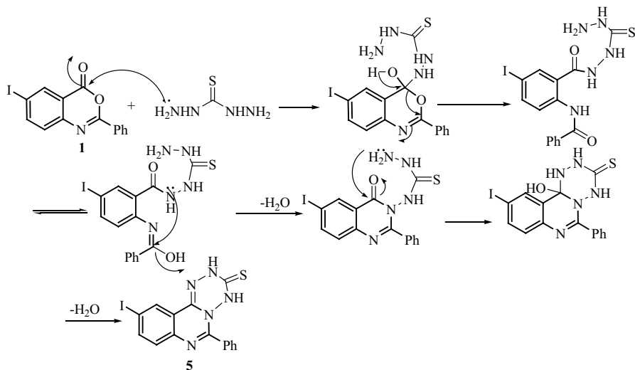
Scheme 2 Proposed mechanism of formation of compound 5
