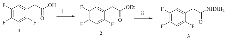
Scheme 1 Synthesis of trifluorophenylacetohydrazide intermediate 3 . Reagents and conditions: (i) \text{EtOH} , \text{H}_2\text{SO}_4 , reflux, 4 h, yield 97%; (ii) \text{NH}_2\text{NH}_2 \cdot 2\text{H}_2\text{O} , \text{EtOH} , reflux, 4 h, yield 70%
