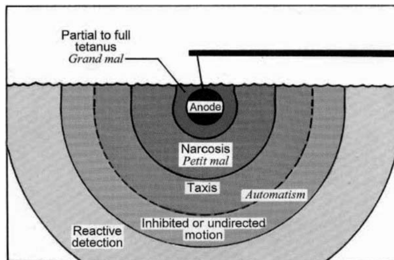
Figure 1. Major intensity-dependent electrofishing response zones. The outer boundaries of response zones for a spherical anode at the surface and sufficiently distant from the cathode are more-or-less hemispherical shells around the anode that represent field-intensity thresholds for the associated responses. Actual and relative sizes of the zones are specimen dependent (species, size, condition, and orientation) and vary with electrical output, electrode size and shape, and environmental conditions. Labels in italics represent corresponding phases of epilepsy as suggested by Sharber and Black (1999) except that here the phase of tonic-clonic contractions (quivering or pseudo-forced swimming) between petit mal and grand mal (narcosis and tetany) is treated as the initial part of grand mal (partial tetany). Zone of reactive detection is sometimes referred to as zone of perception. Zones of taxis, narcosis, and tetany represent the effective range for fish capture using direct and pulsed direct currents. (Reproduced from Snyder (2003), Figure 11.)
