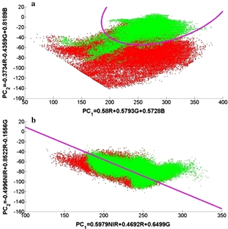
Fig. 5 First (PC1) versus second (PC2) principal components of R, G and B variables (a) and NIR, R and G variables (b) for TSWV-infected and healthy pepper plants. Altogether, 60 000 healthy ( green ) and 60 000 diseased ( red ) pixels are displayed. The pink solid lines represent the functions separating the decision regions (Color figure online)
