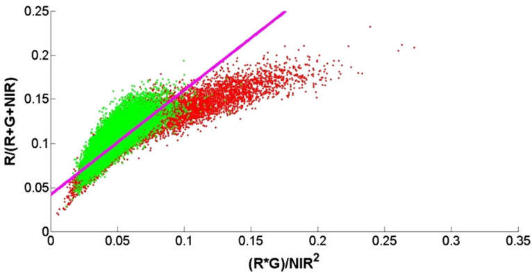
Fig. 7 First index ( R \cdot G / NIR^2 ) versus second index ( R / (R + G + NIR) ) of NIR, R and G variables for PM-infected and healthy pepper plants. Altogether, 20 000 healthy (green) and 20 000 diseased (red) pixels are displayed. The pink solid lines represent the functions separating the decision regions (Color figure online)
