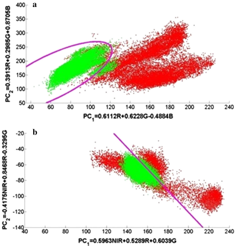
Fig. 6 First (PC1) versus second (PC2) principal components of R, G and B variables (a) and NIR, R and G variables (b) for PM-infected and healthy pepper plants. Altogether, 20 000 healthy (green) and 20 000 diseased (red) pixels are displayed. The pink solid lines represent the functions separating the decision regions (Color figure online)
