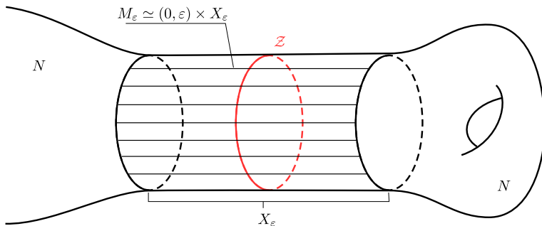
Fig. 1 Tubular neighborhood of the singular region
