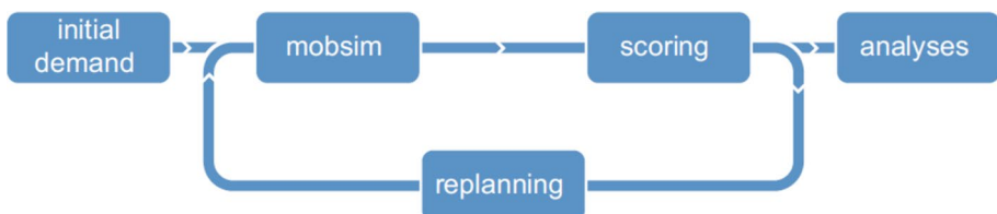
Fig. 1 The overall simulation process in MATSim
