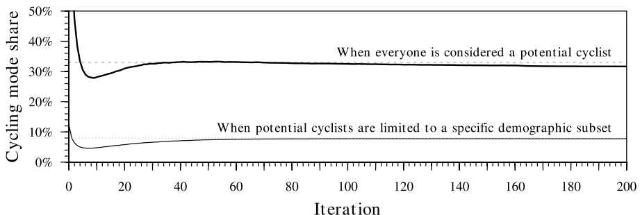
Fig. 3 Convergence in the selection of bicycle plans as the number of model iterations increases
