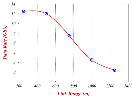
Fig. 8 Data rate per user achievable according to the FSO link
