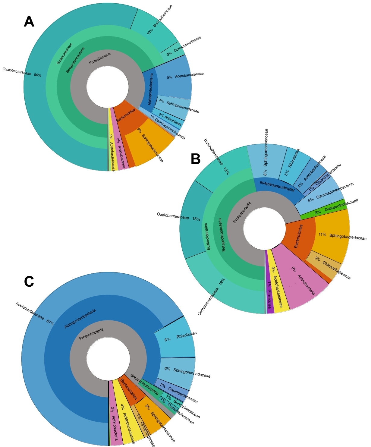
Fig. 2 Relative abundance and taxonomic hierarchy using Krona radial space-filling. (a) Bacterial endophyte community of limber pine seedling shoot tissue, (b) seedling roots, and (c)
