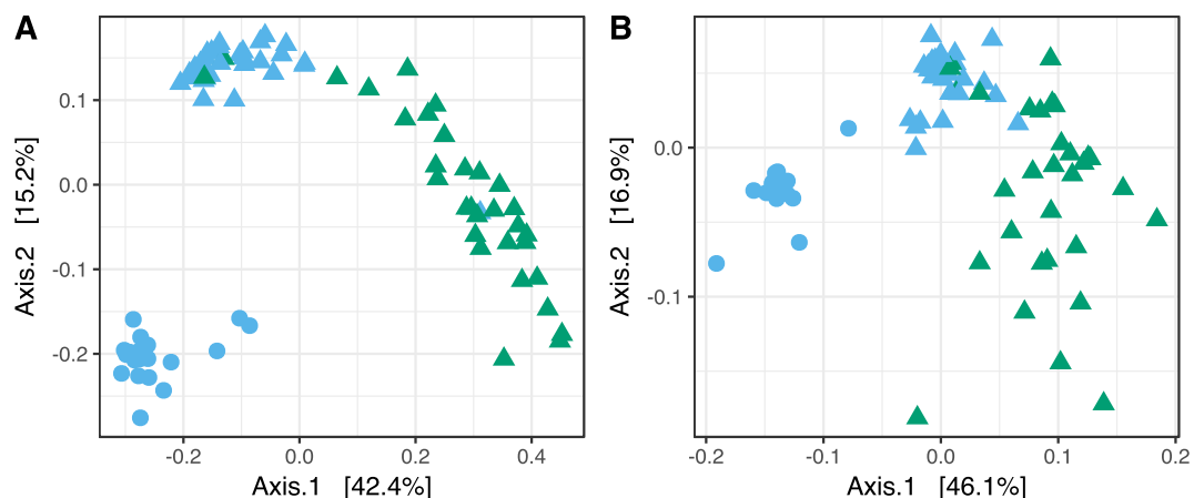
Fig. 1 Principal coordinate analysis showing differentiation between tissue age, shoot and root communities. (a) unweighted and (b) weighted UniFrac distance matrix. Points that are closer together have more similar communities. Each point corresponds to
