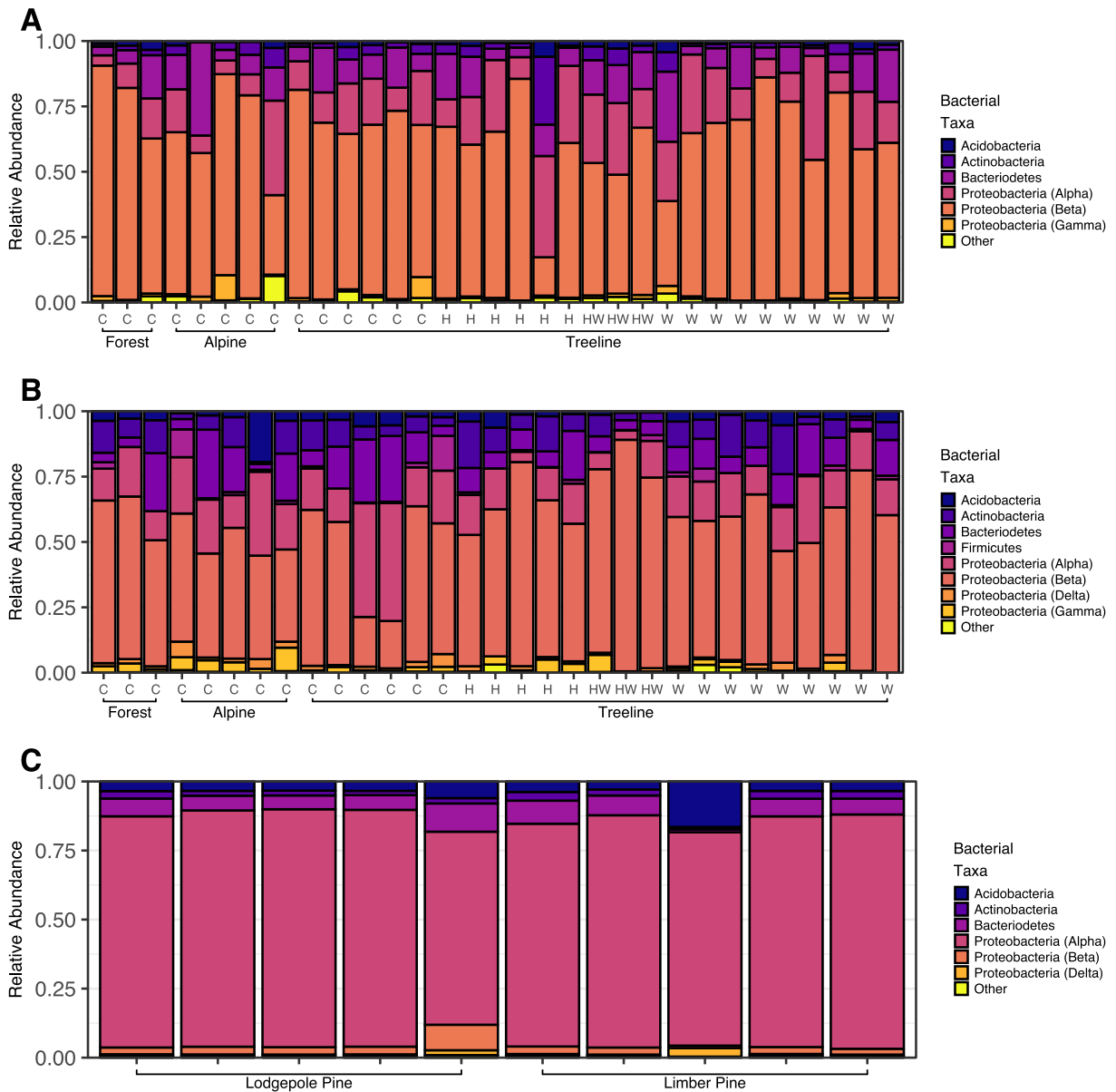
Fig. 3 Relative abundances of the major phyla in seedlings and adult needles as percentages of all of the 16S rRNA gene sequences for (a) shoot tissues, (b) root tissues and (c) mature conifer foliage (both limber pine and lodgepole pine collected in 2012 at
