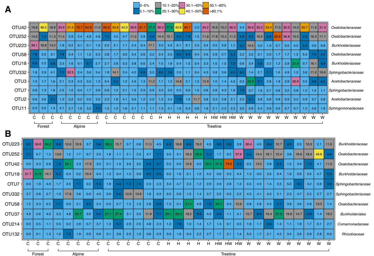
Fig. 4 Heatmap showing the 10 most abundant OTUs and their relative abundances as percentages of all the 16S rRNA gene sequences in each sample. (a) Shoot and (b) root tissues types. Color tones range from warm (orange) to cool (blue) to indicate the highest and lowest abundances. The value in each square is the
