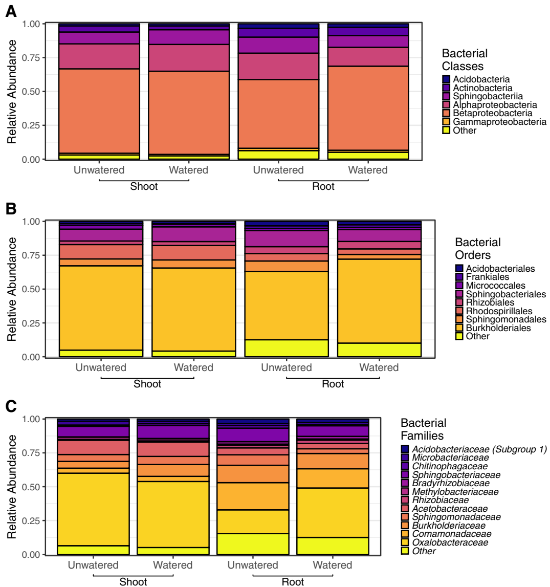
Fig. 5 Bar charts of relative abundances of the major phyla as percentages of the all the 16S rRNA gene sequences grouped by tissue type and watered treatment. (a) Bacterial classes, (b)
