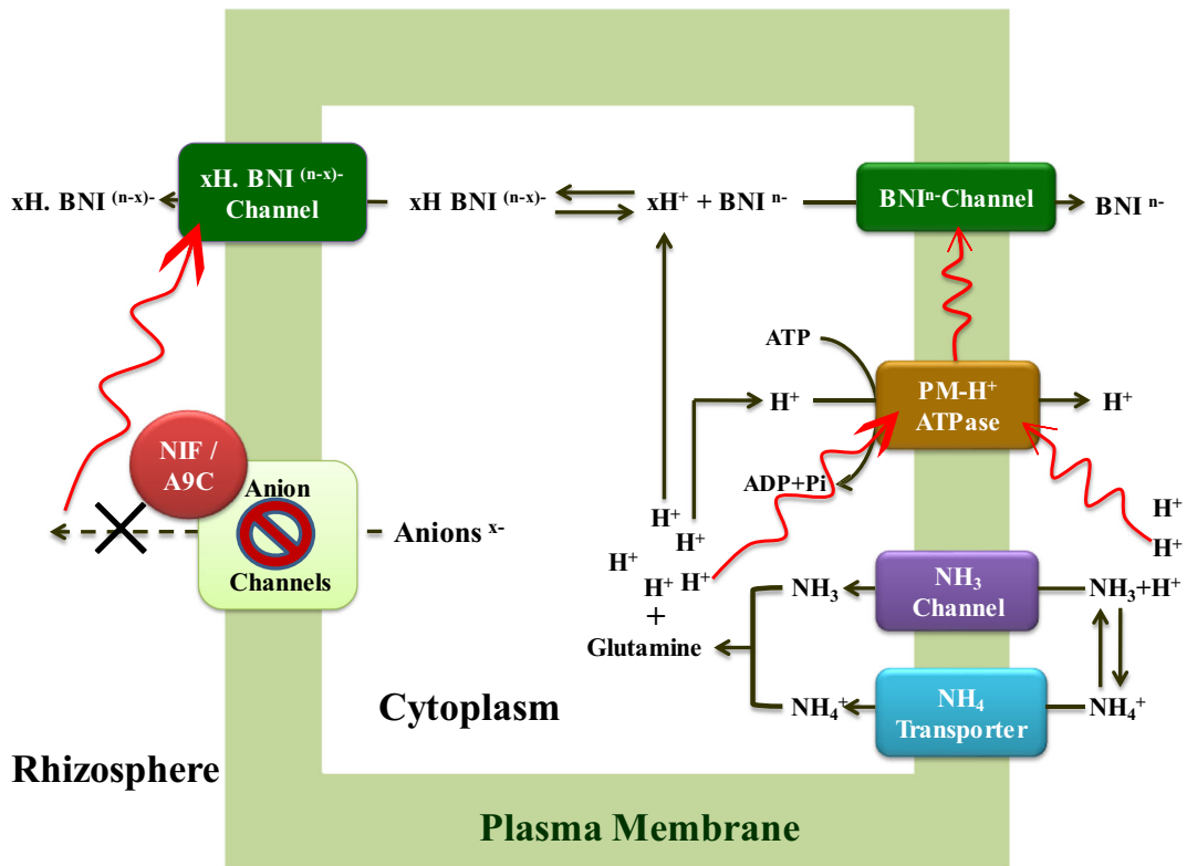
Fig. 11 Proposed new hypothesis for the release of hydrophilic-BNIs in sorghum roots. Schematic description of the BNIs release process; the uptake of ammonium/ammonia causes release of H^+ in rhizosphere, and this triggers PM H^+ ATPase activity, which in turn stimulates release of anionic BNIs through an unknown BNI-channel. In addition, assimilation of ammonium/ammonia in root cells produce H^+ , which needs to be pumped out of the root cells to prevent cytosolic acidification; PM H^+ ATPase can also be activated by cytosolic H^+ , which can regulate hydrophilic-BNIs
