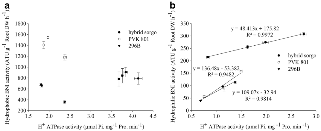
Fig. 7 Relationship between PM H + ATPase activity and hydrophobic BNI activity ( a ) and PM H + ATPase activity and hydrophilic BNI activity in root systems of 3 sorghum genetic stocks – ‘Hybridsorgo’, PVK801 and 296B
