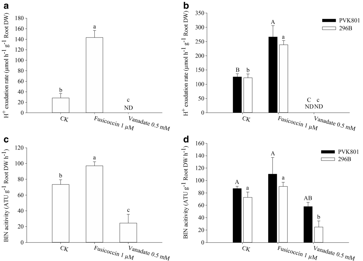
Fig. 8 Influence of fusicoccin and vanadate in root exudate collection solutions on H + exudation rate and hydrophilic-BNIs release in roots of ‘Hybridsorgo’ ( a and c ) and PVK 801 and 296 B
