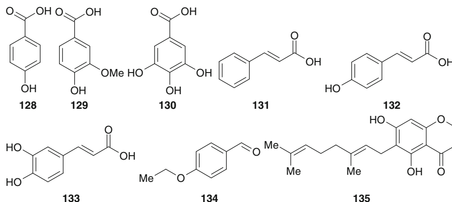
Fig. 7 Miscellaneous compounds
