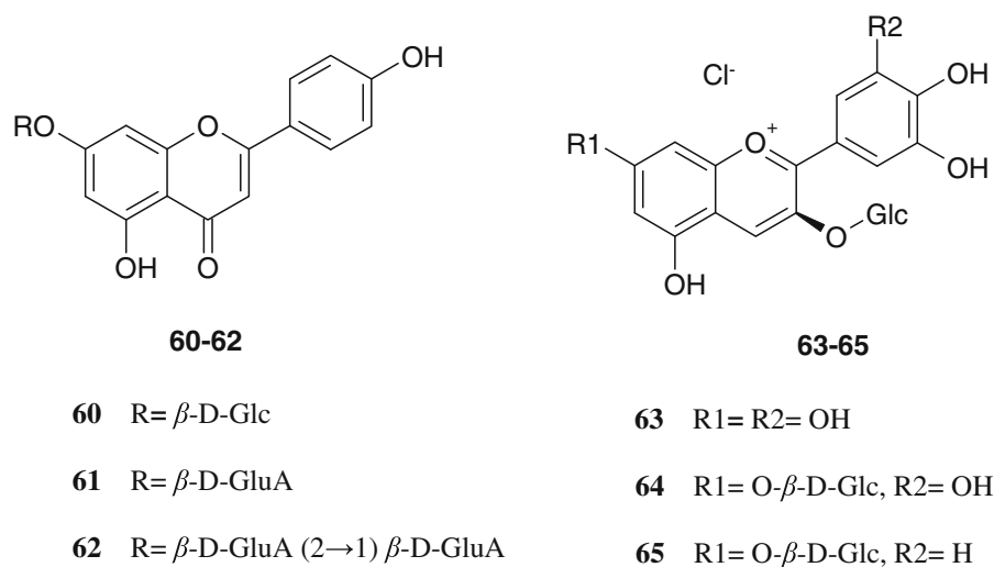
Fig. 2 Flavonoid glycosides
