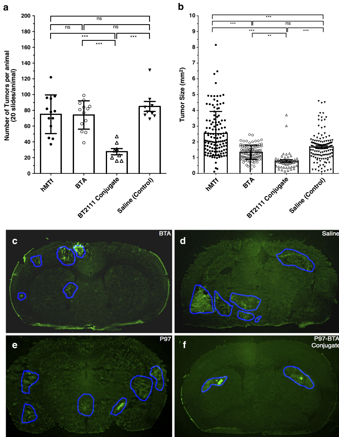
Fig. 4 Number (Fig. 4a) and size (Fig. 4b) of metastatic lesions in the isolated brain of test NuNu mice after administration of saline, P97 (hMTf), BTA and P97-Trastuzumab conjugate (BT2111) biweekly for 2 weeks. The P Value for the number of metastatic lesions for BT2111 vs. control, BTA or hMTf groups was found to be < 0.0001 . Tumor size was based on pooled data from all individual values in each group. The P Value for the size of metastatic lesions for BT2111 vs. control or hMTf groups was found to be < 0.0001 and for BT2111 vs. BTA group was found to be < 0.001 . Figure 4c–f show representative fluorescent images from each group highlighting the metastatic lesions size in the isolated brain of test NuNu mice after administration of saline, hMTf, BTA and BT2111 conjugate biweekly for 2 weeks.
