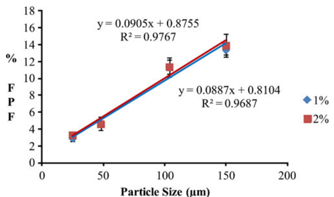
Fig. 9 The relationship between the FPF of SS and the size of the PCL microspheres coated with 1 % and 2 % leucine solution respectively, n=5 .
