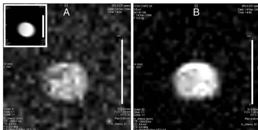
Fig. 13. ^{19}\text{F} MRI spin-echo images of pure PFOB (A, inset, 8 min) and 150 nm capsules suspended in water ( 50 \text{ mg ml}^{-1} : A, 8 min; B, 34 min). Scale bars represent 1 cm (65). Reprinted with permission.
