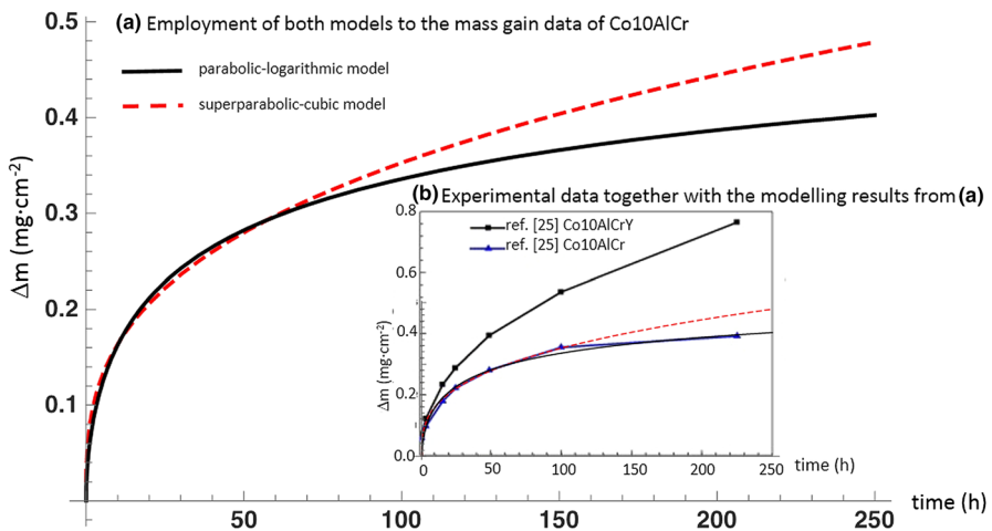
Fig. 10 Comparison of mass gain curves according to parabolic–logarithmic (black line) and superparabolic–cubic (red dashed line) models. Inset: excellent agreement between parabolic–logarithmic model (black line) and experimental observation for CoCrAl at 900 °C [25] k=1 nm/h, r_0=17 nm constant= 0.060 mg 2 /cm 4 , while the superparabolic–cubic model is shown to fail (dashed red line) (Color figure online)
