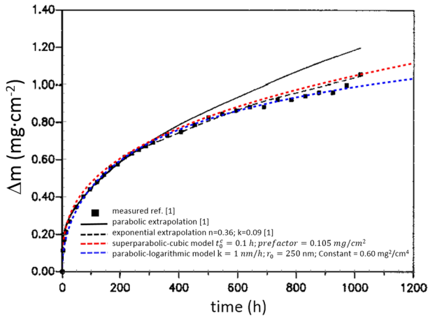
Fig. 9 Comparative analysis of mass gain during oxide growth on MA 956 at 1100 °C. Top: parabolic fit [1]. Red dotted: superparabolic–cubic model, ( t_0^{(3)}=0.1 h, prefactor= 0.105 mg/cm 2 ). Blue dotted: parabolic–logarithmic model for k=1 nm/h, r_0=250 nm, and constant: 0.60 mg 2 /cm 4 (Color figure online)
