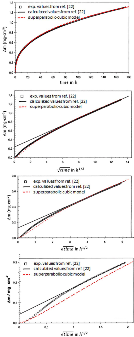
Fig. 5 Deviation from parabolic model for oxide scaling on PM2000 at 1200 °C from [22]. Superparabolic–cubic model (red dashed). Deviation between model and experiment emerges at t < 9 h for t_0^c = 1 h; prefactor = 0.245 mg/cm 2 (Color figure online)
