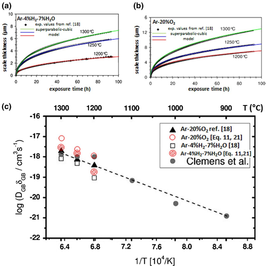
Fig. 6 Exposures in Ar-4%H 2 -7% H 2 O as well as in Ar-20%O 2 at 1200, 1250 and 1300 °C [18] are described, respectively, by the superparabolic–cubic model for prefactors and t_0^c in parentheses, a 0.7 μm (0.60 h); 1.35 μm (0.40 h); 1.7 μm (1.10 h), and b 1.55 μm (0.05 h); 2.00 μm (0.40 h); 3.03 μm (1.4 h). c \delta_{GB}D_{GB} values are obtained from Eq. 11, (red symbols) by employing \frac{\Delta x}{RT} data from Ref. 18 (Color figure online)
