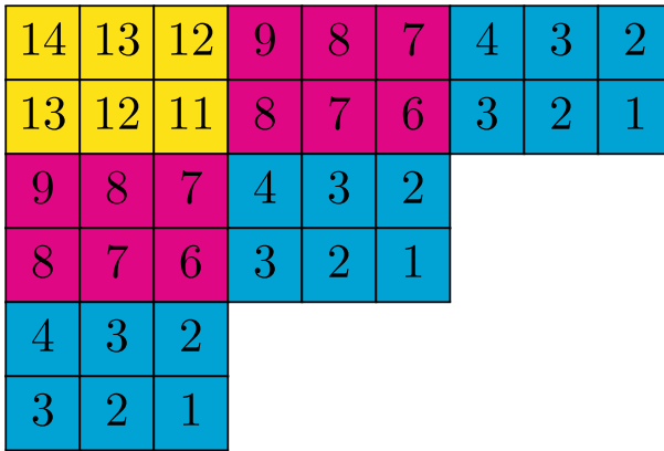
Fig. 4 The filling H of the Ferrers diagram \lambda(\beta) for \beta generating \mathbf{BL}(3^4) , partitioned into rectangles of size 2 \times 3
