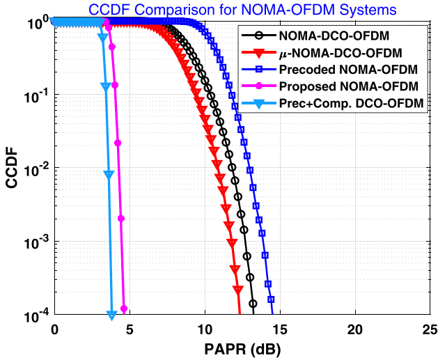
Fig. 2 PAPR comparison for different NOMA DCO-OFDM systems
