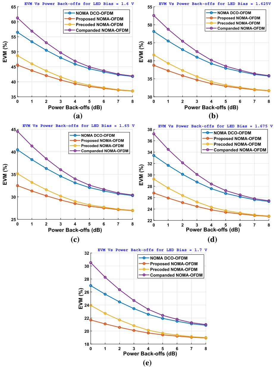
Fig. 4 Mean EVM comparison for different LED bias voltages a LED bias = 1.6 V, b LED bias = 1.625 V, c LED bias = 1.65 V, d LED bias = 1.675 V and e LED bias = 1.7 V
