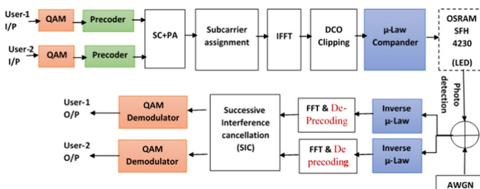
Fig. 1 Transceiver of the proposed NOMA DCO-OFDM system
