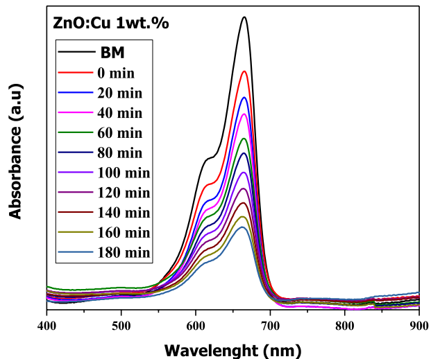
Fig. 7 The absorption spectra of MB for the 1 wt% Cu doped ZnO film
