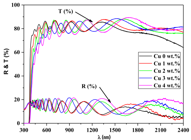
Fig. 3 Optical transmission and reflectance of Cu-doped ZnO thin films at various CuContents
