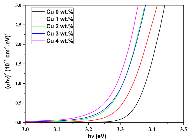
Fig. 4 The plots of (ah\nu)^2 against h\nu of Cu-doped ZnO thin films at various Cu contents
