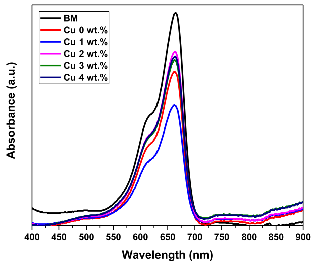
Fig. 8 Absorption spectra of MB after solar irradiation for 3 h using the Cu doped ZnO thin films at various Cu contents
