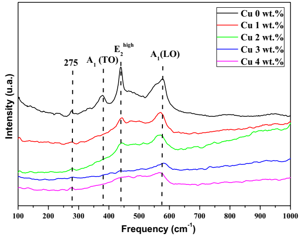
Fig. 2 Raman scattering spectra of the Cu doped ZnO films at various Cu contents
