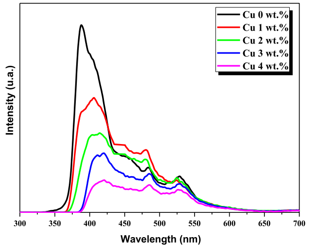
Fig. 6 PL spectra of undoped and Cu-doped ZnO films at various Cu contents
