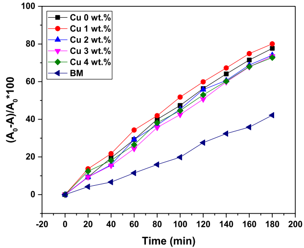
Fig. 9 The degradation efficiencies of MB dye versus irradiation time
