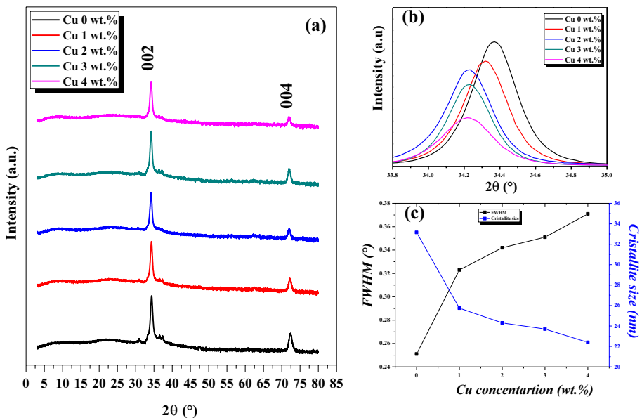
Fig. 1 X-ray diffraction (XRD) patterns of the Cu doped ZnO thin films at various Cu contents (a), the enlarging XRD patterns of the (002) plane peak (b), the variation of FWHM and crystalline size at various Cu contents (c)
