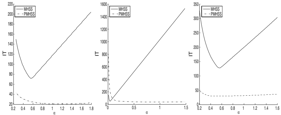
Fig. 2 Pictures of IT versus \alpha for MHSS and PMHSS iteration methods with m = 64 ; left: Example 4.1, middle: Example 4.2, and right: Example 4.3
