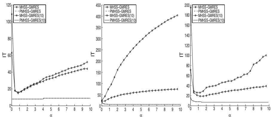
Fig. 3 Pictures of IT versus \alpha for MHSS- and PMHSS-preconditioned GMRES(10) and GMRES methods; left: Example 4.1, middle: Example 4.2, and right: Example 4.3
