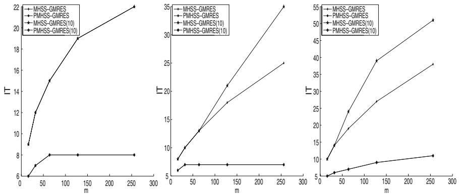
Fig. 1 Pictures of IT versus m for MHSS- and PMHSS-preconditioned GMRES(10) and GMRES methods with \alpha = \alpha_{exp} ; left : Example 4.1, middle : Example 4.2, and right : Example 4.3
