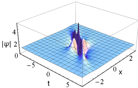
Fig. 7 The second-order rogue wave, Eqs. (18), (19), (20), obtained from the degenerate 2-breather solution shown in Fig. 6 in the limit \kappa \rightarrow 0 , with some stretching due to higher-order effects
