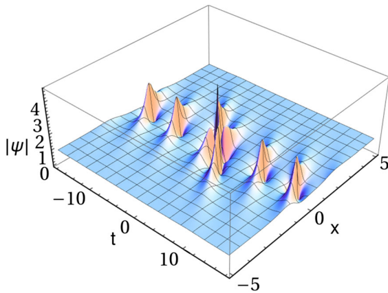
Fig. 5 The 2-breather solution in the semirational limit. Here the nonzero modulation parameter is \kappa = 1 , with \alpha_n the same as in Fig. 1. It can be considered as a superposition of the Akhmediev breather with the Peregrine solution
