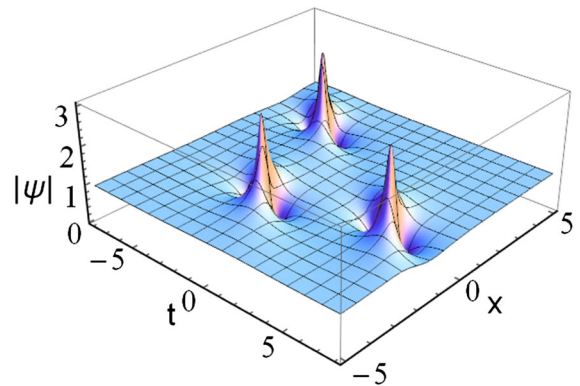
Fig. 8 The second-order rogue wave triplet (21), with separation parameters \xi = -\eta = 480 , and the extended equation parameters given by \alpha_2 = \frac{1}{2} , \alpha_3 = \frac{1}{27} , \alpha_4 = \frac{1}{50} , \alpha_5 = \frac{1}{81} , \alpha_6 = \frac{1}{200} , \alpha_7 = \frac{1}{343} . For this choice of parameters, we have B = \frac{77}{50} , v = \frac{1324}{1323} , B'' = -\frac{7}{25} and v'' = -\frac{2894}{3969}
