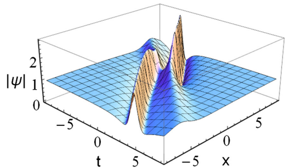
Fig. 10 The second-order rogue wave solution with ‘soliton’-like tails when B = 0 , but now \xi = \eta = 48
