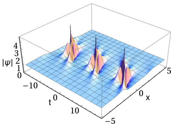
Fig. 1 The 2-breather solution (6) of Eq. (1). The modulation parameters are at a ratio \kappa_1 : \kappa_2 = 1 : 2 . Parameters of the equation are: \alpha_2 = \frac{1}{2} , \alpha_3 = \frac{1}{6} , \alpha_4 = \frac{1}{24} , \alpha_5 = \frac{1}{30} , \alpha_6 = \frac{1}{144} , with all higher \alpha_n = 0 . The wave profile is tilted in the (x, t) -plane due to the nonzero v_m
