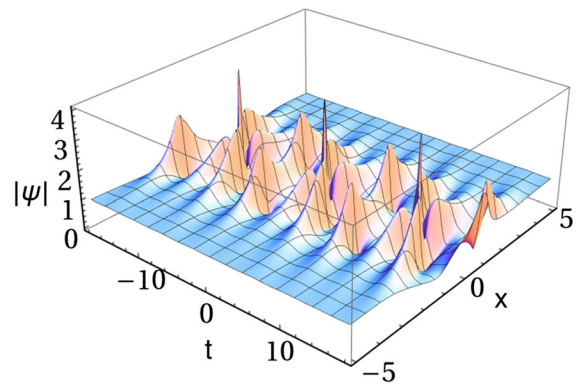
Fig. 3 The 2-breather solution with \alpha_n = 1/n! up to n = 8 , with all higher \alpha_n = 0 , but now with \kappa_1 = \frac{3}{2} , and \kappa_2 = 1
