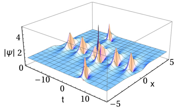
Fig. 2 A collision between an Akhmediev breather and Kuznetsov–Ma soliton, with \kappa_1 = 1 , and \kappa_2 = i . Here \alpha_n = 1/n! up to n = 8 , with all higher \alpha_n = 0
