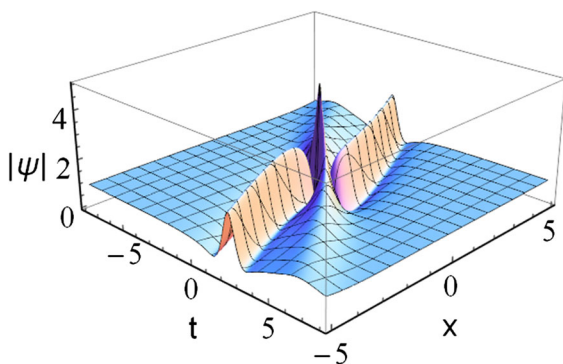
Fig. 9 The second-order rogue wave solution with ‘soliton’-like tails when \alpha_2 is chosen such that B = 0 , and \xi = \eta = 0 . Other parameters are the same as in Fig. 8
