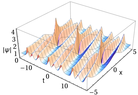
Fig. 4 A wave profile of a ‘breather-to-soliton conversion.’ We use the same set of parameters as in Fig. 3, except \alpha_2 is now chosen such that B_2 = 0 . This choice extends to infinity the tails of the breathers that would otherwise decay
