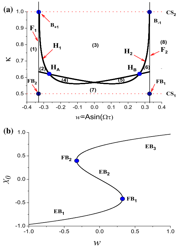
Fig. 2 Bifurcations for \alpha = 8.0, \beta = 0.5, \gamma = 8.0, \delta = -0.15, b = -2.0, c = 0 . a Bifurcation sets on the (\kappa, w) plane b equilibrium branches with the variation of w
