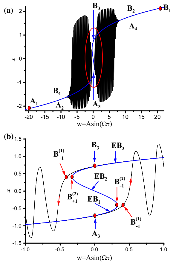
Fig. 12 a Overlap of the transformed phase portrait and the equilibrium branches b Locally enlarged of the overlap
