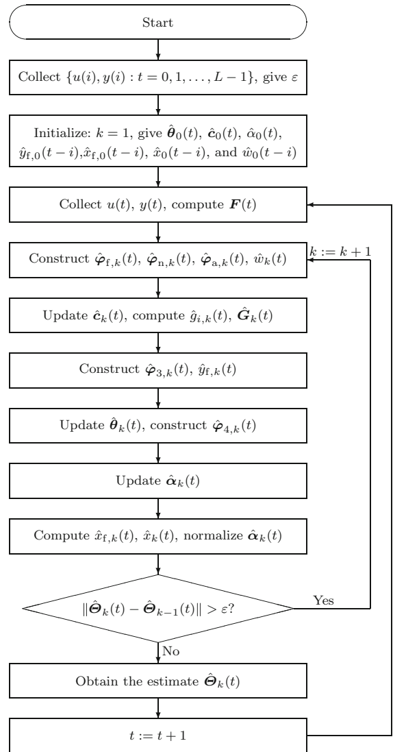
Fig. 2 The flowchart of the F-D-LSI algorithm for computing \hat{\boldsymbol{\theta}}_k(t) , \hat{\boldsymbol{\alpha}}_k(t) and \hat{\mathbf{c}}_k(t)
