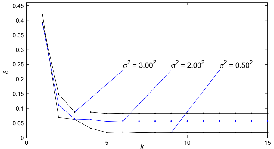
Fig. 6 The F-D-LSI estimation errors \delta versus k ( L = 2000 )
