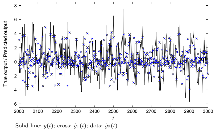
Fig. 9 The true output and predicted output from t = 2001 to 3000 ( \sigma^2 = 1.00^2 , k = 15 )
