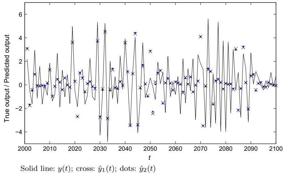
Fig. 8 The true output and predicted output from t = 2001 to 2100 ( \sigma^2 = 1.00^2, k = 15 )
