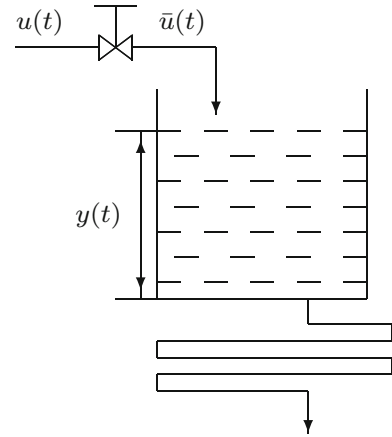
Fig. 4 An experimental setup of a water tank system
