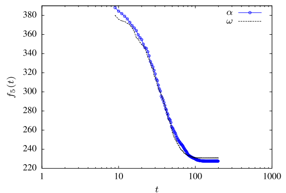
Fig. 10 Evolution of the Rastrigin function, with variable \alpha and \omega
