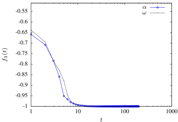
Fig. 8 Evolution of the Drop wave function, with variable \alpha and \omega
