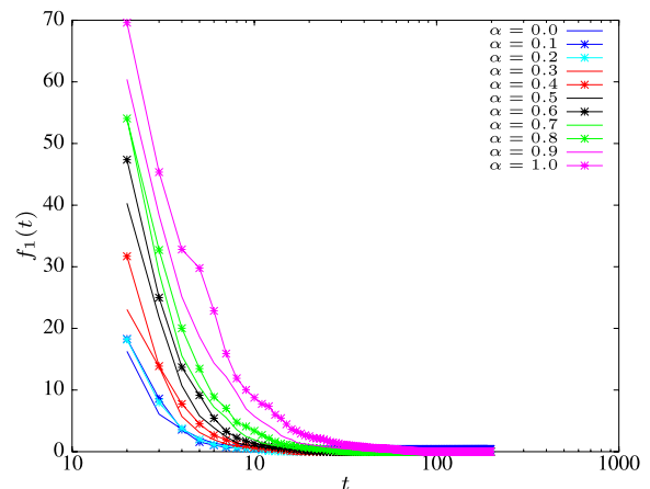
Fig. 1 Evolution of the Bohachevsky 1 function for \alpha = \{0, \dots, 1\} , with best value of \alpha = 0.19
