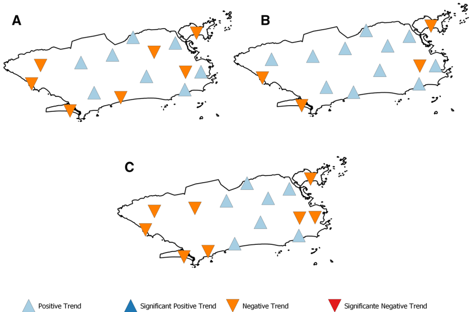
Fig. 3 Climate change indices trend in Rio de Janeiro City: a Rx1day, b Rx5day, c R99p
