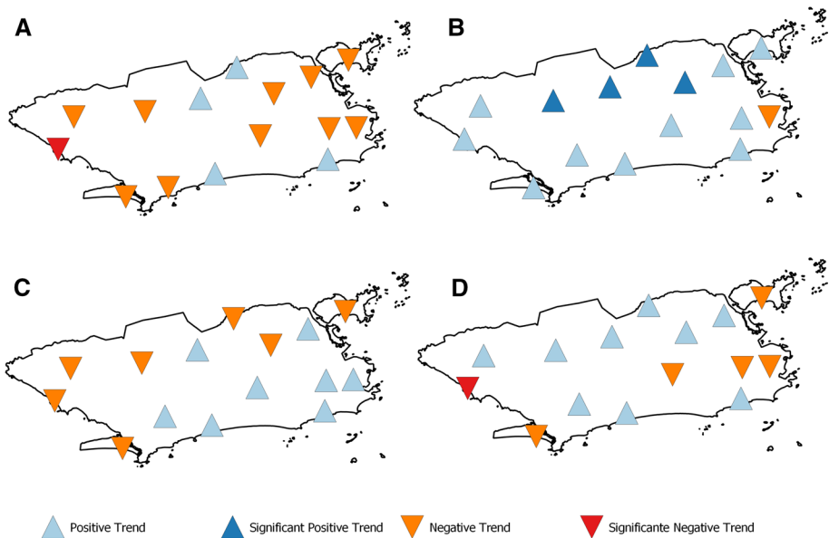
Fig. 2 Climate change indices trend in Rio de Janeiro City: a PRCPTOT, b CDD, c CDW and d DSII
