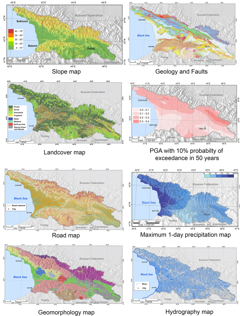
Fig. 7 Factor maps used in the landslide susceptibility assessment. For the geological and geomorphological maps, no legends can be shown as there are too many units. Higher-resolution maps with complete legends can be downloaded from: http://drm.cenn.org/paper_atlas/RA-part-2.pdf
