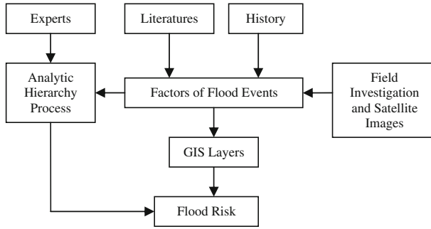
Fig. 4 Research methodology
