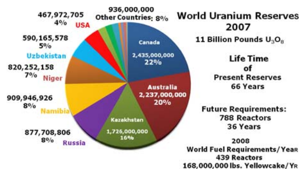
Figure 6. World Uranium reserves (Source: International Atomic Energy Agency, http://www.iaea.org/ ).
