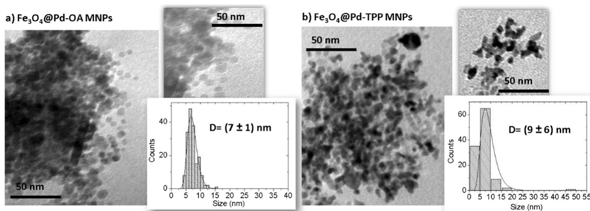
Fig. 3 TEM micrographs for core-shell \text{Fe}_3\text{O}_4 @Pd-OA (a) and \text{Fe}_3\text{O}_4 @Pd-TPP (b)
