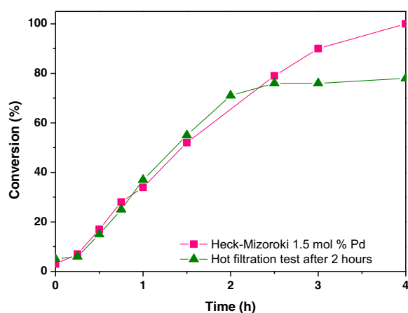
Fig. 5 Hot filtration test in Heck-Mizoroki coupling reaction between p -iodoanisole and styrene catalyzed by Fe 3 O 4 @Pd-OA catalyst
