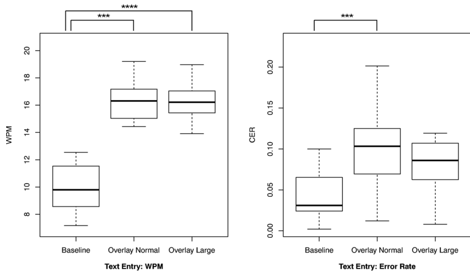
Fig. 6 WPM (left) and CER (right) scores across conditions (* p < 0.05 ** p < 0.01 *** p < 0.005 **** p < 0.001 )
