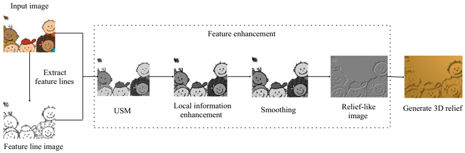
Fig. 1 Framework of our algorithm
