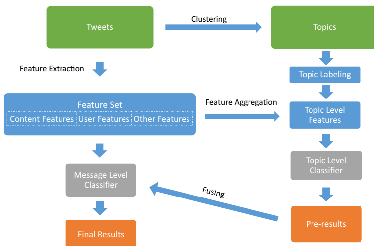
Fig. 5 Overview of the MCG-ICT two-level classification model. Topic-level classifications are fused with the message-level ones to produce the final result
