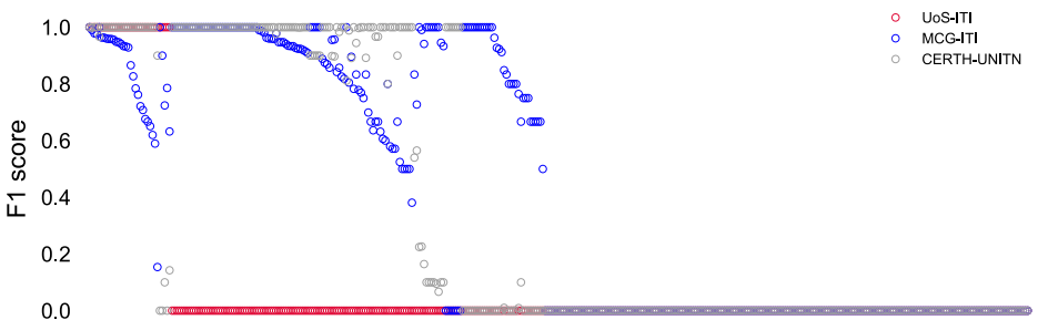
Fig. 10 F1 -score across unique images for each approach. To make the visualization of results cleaner, images in the x axis are sorted based on the mean F1 -score across the three approaches
