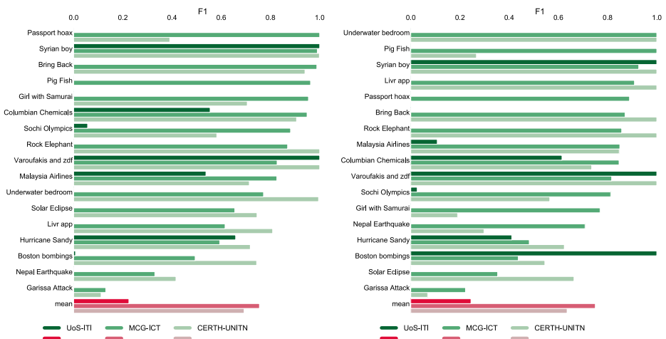
Fig. 8 F1 -scores for dataset#1 and dataset#2 per event and approach
