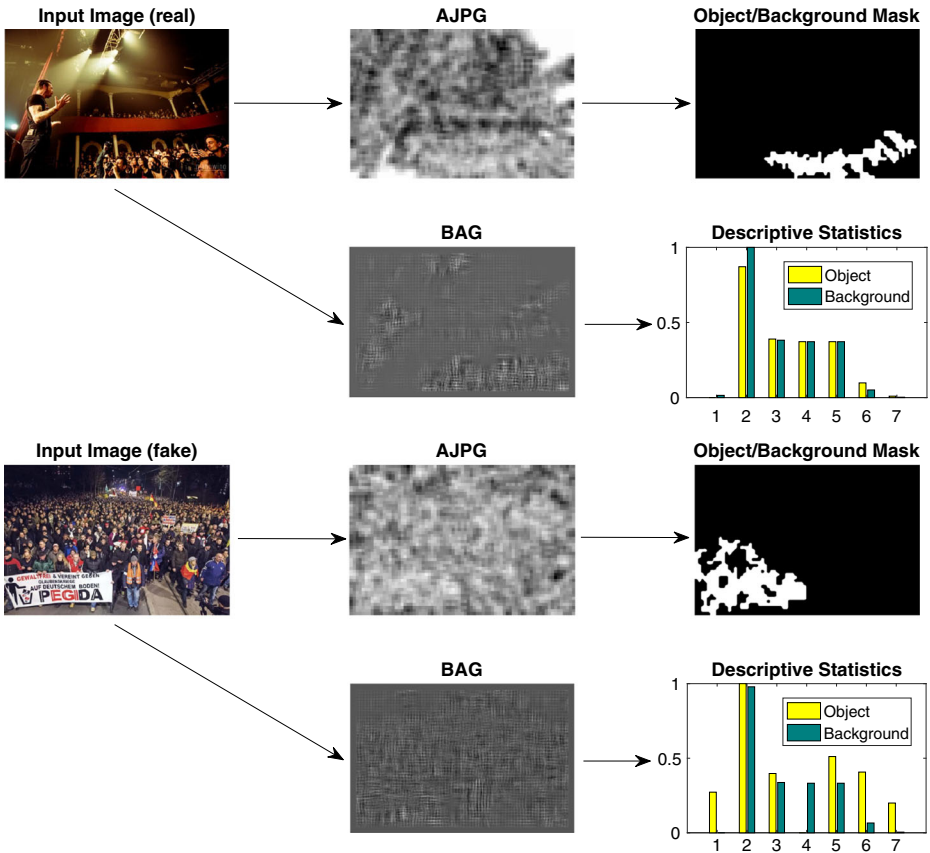
Fig. 7 Illustration of forensics feature extraction process
