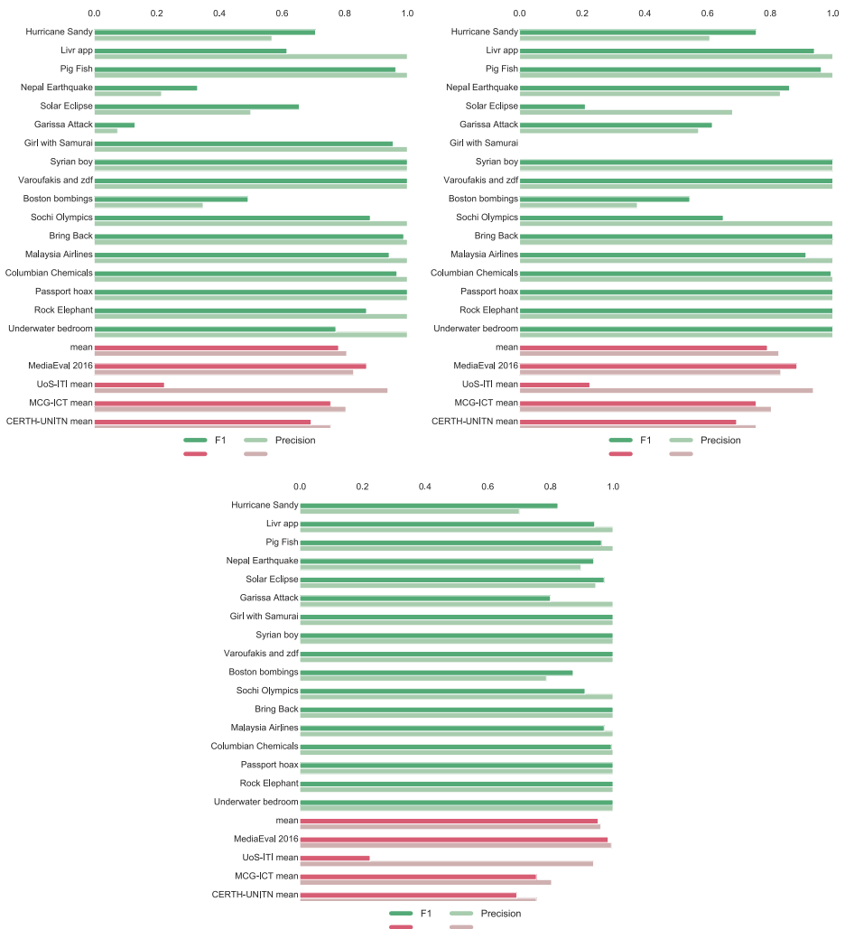
Fig. 11 F1-scores and Precision of the ENS-MAJ, ENS-HPF and ENS-ORA ensemble methods for dataset#1, mean score of each method on the dataset of MediaEval '16 and individual mean scores of the approaches
