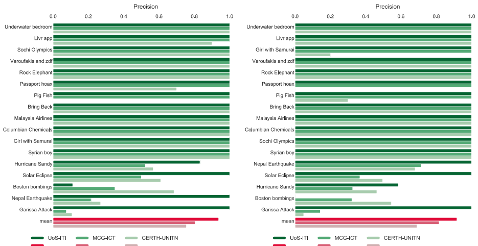
Fig. 9 Precision scores for dataset #1 and dataset #2 per event and approach
