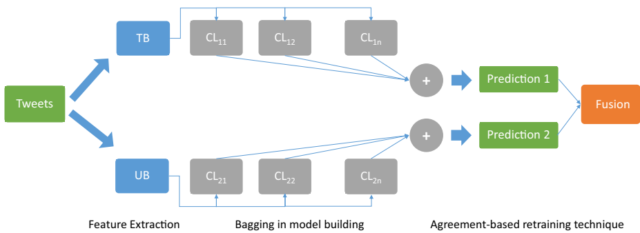
Fig. 6 Overview of the CERTH-UNITN method
