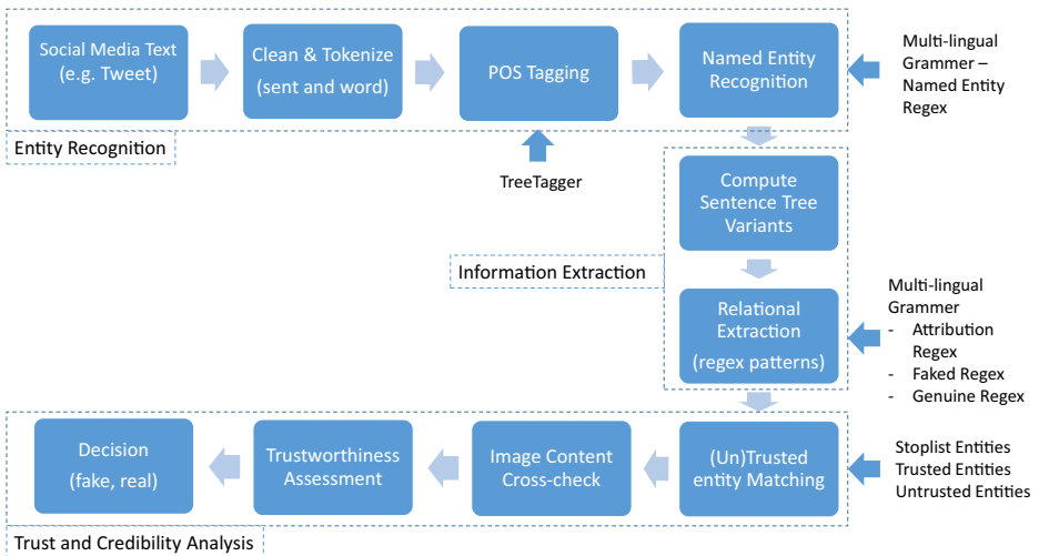
Fig. 4 NLP pipeline for regex-based NER and RE in UoS-ITI
