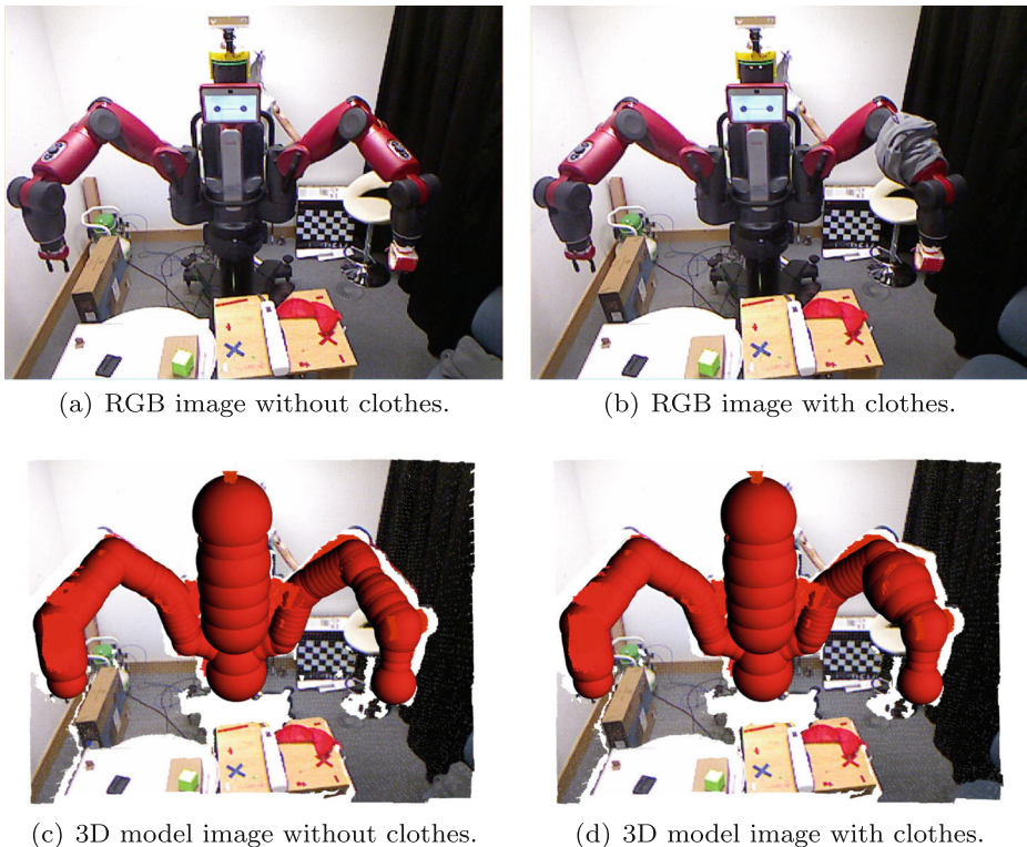
Fig. 13 Self-Identification results with and without clothes on the left arm
