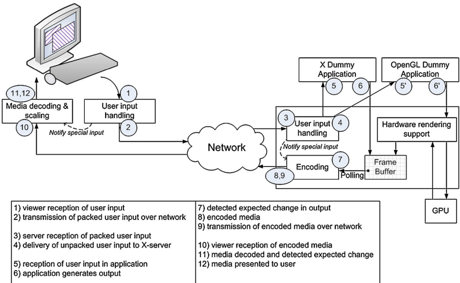
Fig. 2 Interception points where timestamps are taken, enabling a breakdown of the interactivity evaluation
